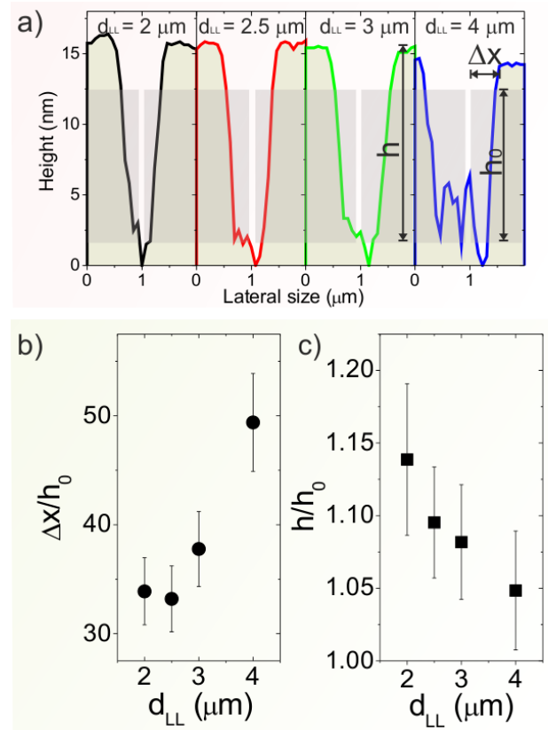
FIG. 4. a) Height profile obtained from AFM images of parallel trenches etched by FIB after dewetting. An example of the AFM image showing the full patch width is provided in the S.I. From the left to the right panel d_{LL} = 2, 2.5, 3, and 4 \mu\text{m} . Shaded areas highlight the original shape of the UT-SOI before annealing. h_0 highlights the original film height and h its final height. \Delta x is a measure of the edge retraction distance from its original position before dewetting. b) Retraction distance \Delta x (in unity of h_0 ) as a function of d_{LL} . c) Film height h (in unity of h_0 ) as a function of d_{LL} . h , x and the experimental errors are determined as average values and standard deviations over ten measurements. See also the S.I.
