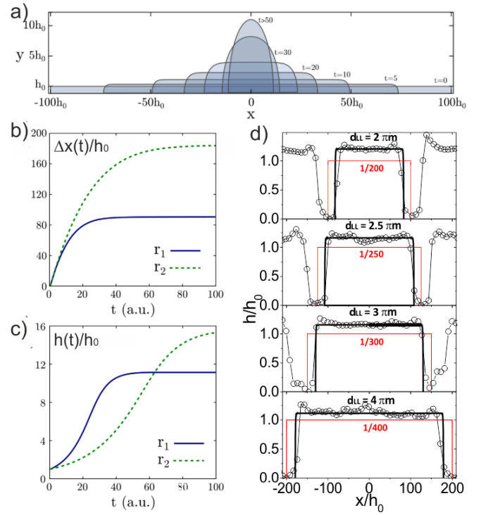
FIG. 7. a) Representative stages of the evolution by SALK of a rectangle (the cross section of a stripe) with height-to-base aspect ratio r_1 = 1/200 . Time is expressed in arbitrary units. Simulation are performed with h_0 = 1 . b) Edge displacement over time for patches with r_1 = 1/200 and r_2 = 1/400 . c) Thickening over time for profiles with r_1 and r_2 (see also video S.V.1). d) Comparison between experimental and theoretical profiles. The red curve represents the initial condition of the UT-SOI before annealing, the black line the film at t = 4 and the symbols are the experimental data (see also the S.I.).
