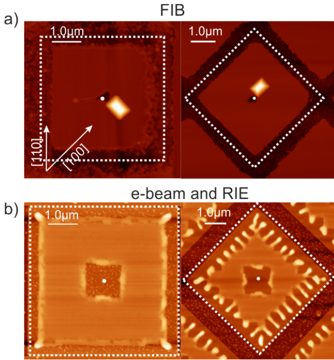
FIG. 3. a) Left (Right) panel: square patch etched via FIB after annealing oriented along the [110] ([100]) crystallographic direction. The white dashed square highlights the original shape of the patch before annealing. In both cases, sub-micrometric, rectangular island is formed next to the central hole after annealing. b) Left (Right) panel: square patch etched via e-beam lithography and reactive ion etching oriented along the [110] ([100]) crystallographic direction after annealing. The white dashed square highlights the original shape of the patch before annealing. See reference [13] for more details on this case.
