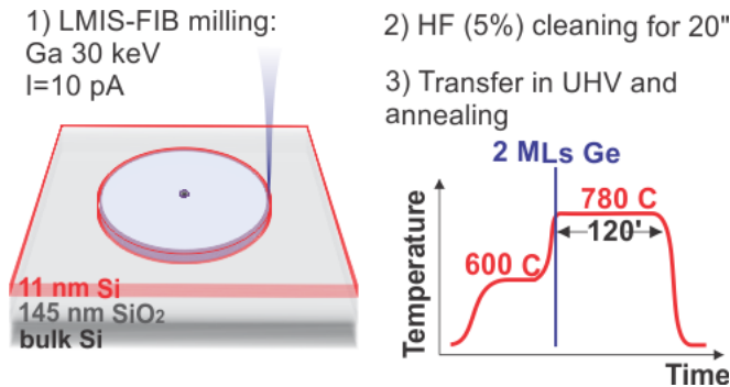
FIG. 1. 1) scheme of the UT-SOI (initial thickness h_0 = 11 nm thick UT-SOI atop 145 nm thick buried oxide, BOX) and liquid-metal ion-source focused ion beam used to mill free patterns (e.g. trenches, squares, circles, pits, etc); 2) removal of native oxide via wet-etching; 3) annealing in the ultra-high vacuum (UHV) of a molecular beam epitaxy reactor. First the samples are annealed at 600°C for 30 minutes followed by deposition of 2 monolayers of Ge and finally annealed at 780°C for 120 minutes.
