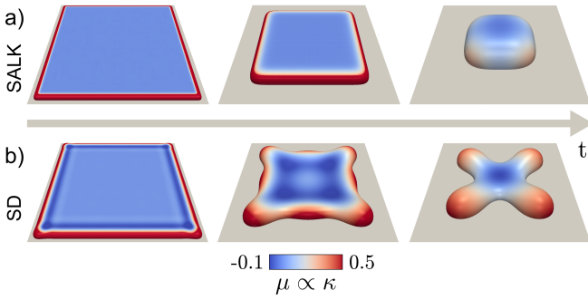
FIG. 6. a) 3D phase-field simulations reproducing the dewetting by SALK of a patch having aspect ratio 1/40. b) Same as a) for SD dynamics (for more details on this case see Ref. [13]).
