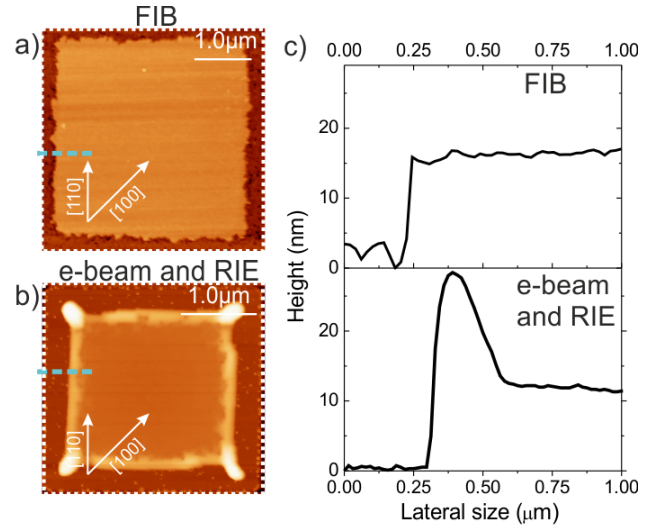
FIG. 2. a) Square patch etched via FIB after annealing. The white dashed square highlights the original shape of the patch before annealing. b) Square patch etched via e-beam lithography and reactive ion etching (e-beam and RIE) after annealing (see reference [13] for details). The white dashed square highlights the original shape of the patch before annealing. c) Comparison between the patch edge profile after annealing for both FIB (top panel) and e-beam and RIE (bottom panel) etching extracted from a) and b) (highlighted by dashed lines).
