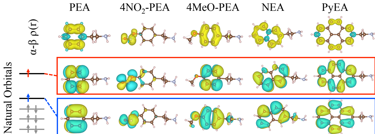
Figure 2: Spin density of the triplet state (top row) and natural orbitals of the open shell states in selected organic spacer candidates.
