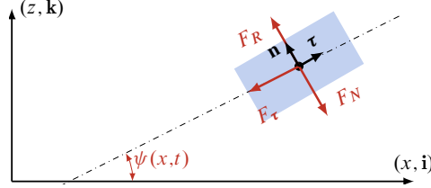
Figure 2: Schematic of the forces acting on a generic infinitesimal element of the plate.
