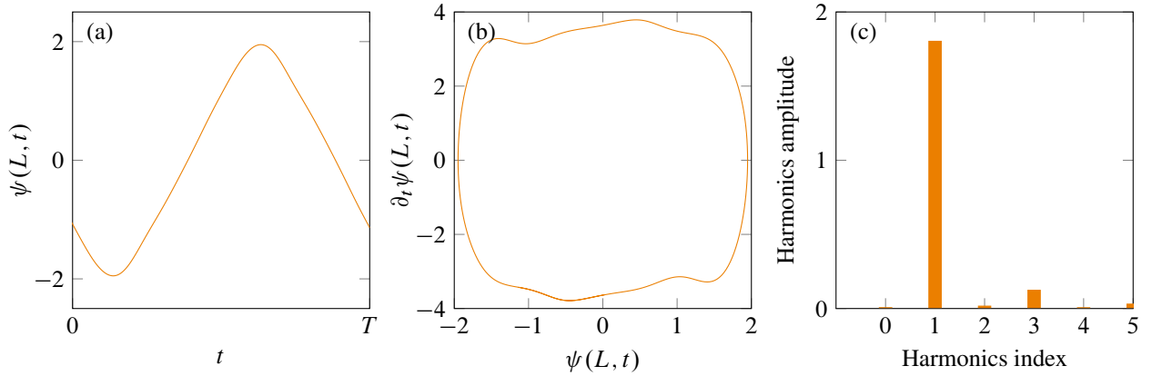
Figure 5: Periodic response of the inverted flag with \mu = 0.3 and \mathcal{R} = 0.5 at \Pi = 6.0 displaying a periodic motion around the trivial equilibrium; (a) time history, (b) phase-plane portrait, (c) and FFT plot indicating the frequency content of the response. Colour scheme from Figure 4(a).
