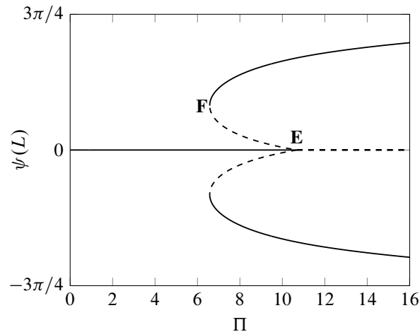
Figure 12: Bifurcation diagram of the inverted flag with \mu = 0.0 and \mathcal{R} = 0.5 . [—] Stable static solution (undeflected stable equilibria), [-.-] unstable static solution.
