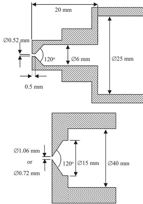
Figure 1. Nozzle scheme.
