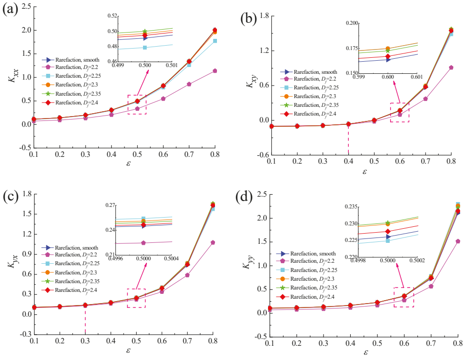
Figure 14. Effect of eccentricity ratio on dynamic stiffness coefficients with different fractal dimensions. (a) K_{xx} vs. \epsilon ; (b) K_{xy} vs. \epsilon ; (c) K_{yx} vs. \epsilon ; (d) K_{yy} vs. \epsilon .
