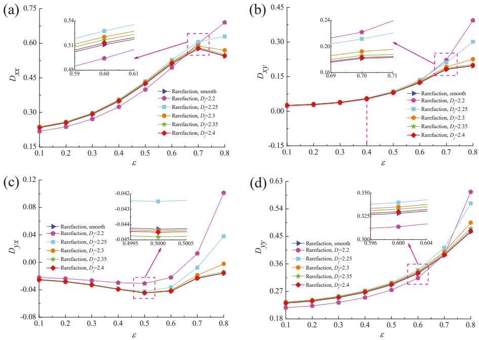
Figure 15. Effect of eccentricity ratio on dynamic damping coefficients with different fractal dimensions. (a) D_{xx} vs. \varepsilon ; (b) D_{xy} vs. \varepsilon ; (c) D_{yx} vs. \varepsilon ; (d) D_{yy} vs. \varepsilon .
