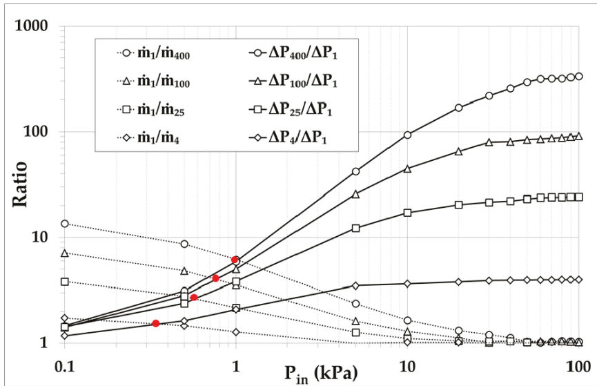
Figure 4. Ratios of total maximum mass flow rates \dot{m}_1 / \dot{m}_n and associated maximum pressure differences \Delta P_n / \Delta P_1 for various one-stage layouts (numbers of microchannels n = 4, 25, 100, 400 and corresponding diameters d = 50, 20, 10, 5 \mu\text{m} ) compared to the reference layout ( n = 1, d = 100 \mu\text{m} ).
