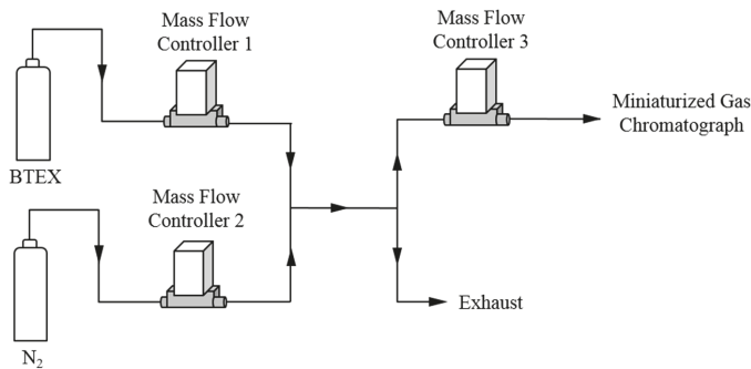
Figure 3. Experimental setup for BTEX generation.
