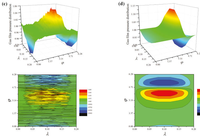
Figure 5. Pressure distributions and contour plots of the gas-lubricated microbearing for different bearing numbers and eccentricity ratios: (a) \epsilon = 0.6 , \Lambda = 20 , D_f = 2.3 , and G = 1 \times 10^{-10} m, (b) \epsilon = 0.6 , \Lambda = 60 , D_f = 2.3 , and G = 1 \times 10^{-10} m, (c) \epsilon = 0.3 , \Lambda = 20 , D_f = 2.3 , and G = 1 \times 10^{-10} m, and (d) \epsilon = 0.6 , \Lambda = 20 , smooth.
