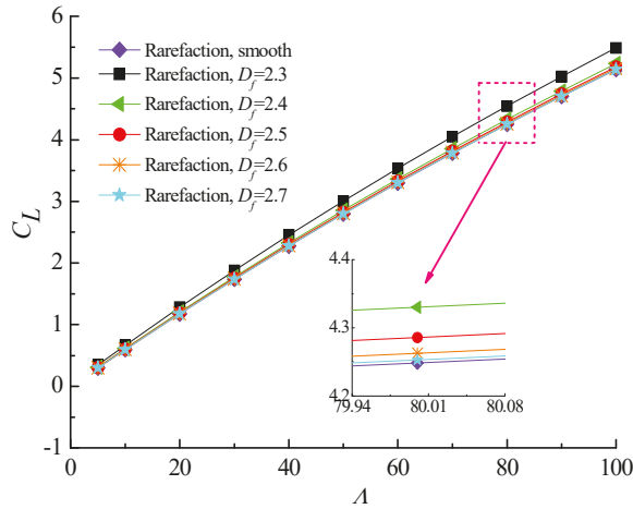
Figure 9. Non-dimensional load capacity versus bearing number for different fractal dimensions at \varepsilon = 0.6, G = 1 \times 10^{-10} .
