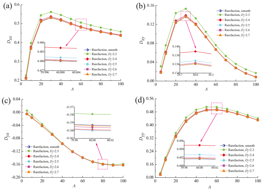
Figure 17. Effect of bearing number on dynamic damping coefficients with different fractal dimensions. (a) D_{xx} vs. \Lambda ; (b) D_{xy} vs. \Lambda ; (c) D_{yx} vs. \Lambda ; (d) D_{yy} vs. \Lambda .
