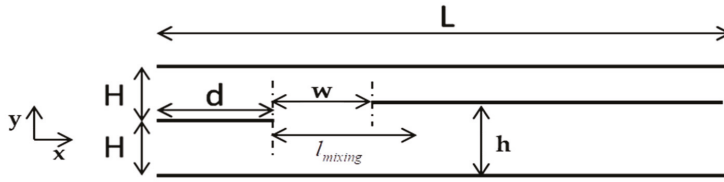
Figure 2. Schematic of gas micro-mixer with splitter.
