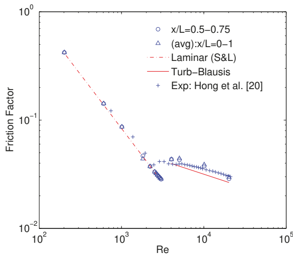
Figure 5. Numerical validation of friction factor calculation.
