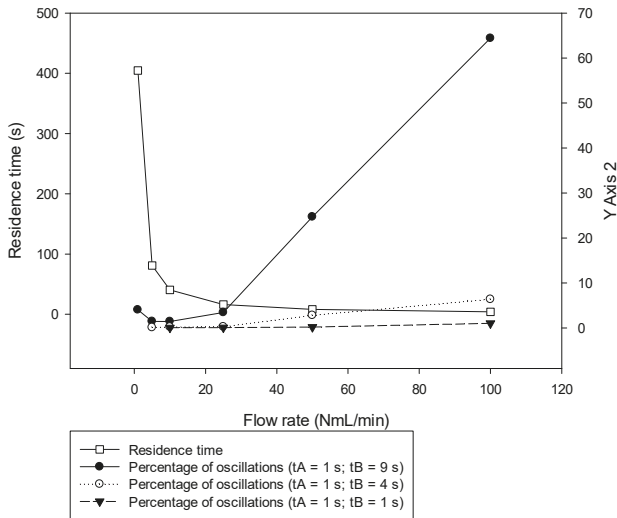
Figure 6. Residence time and percentage of oscillations around the targeted scalar 0.1 for flow rates ranging from 1 to 100 NmL·min -1 at the exit of the 4th mixing stage. Percentage of oscillations is given for t_A = 1 s and t_B = 9 s, 4 s and 1 s.
