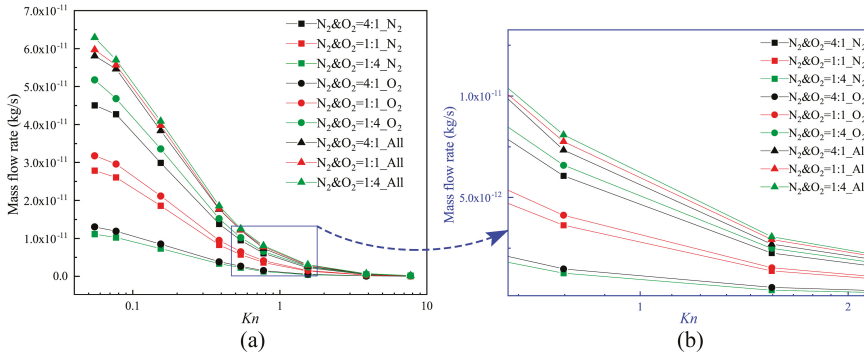
Figure 8. Mass flow rates for different Knudsen numbers.
