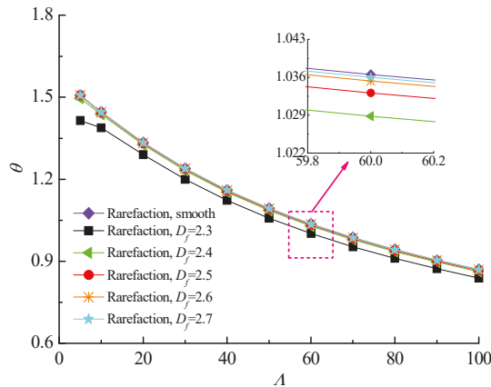
Figure 10. Attitude angles versus bearing number for different fractal dimensions at \varepsilon = 0.6, G = 1 \times 10^{-10} .
