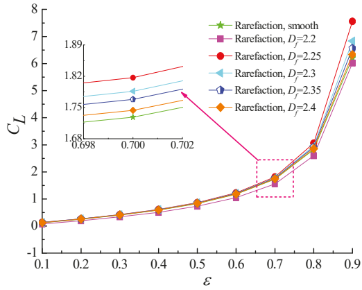
Figure 6. Non-dimensional load capacity versus eccentricity ratio for different fractal dimensions at \Lambda = 20, G = 1 \times 10^{-11} .
