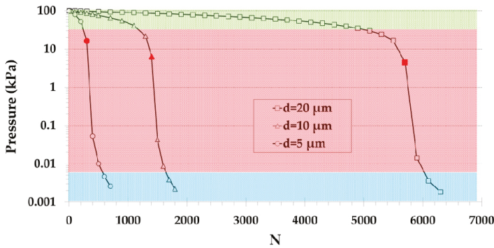
Figure 8. Inlet pressure evolution of a system connected to pump B as a function of its number of stages, considering narrow diameter channels d = 5, 10, 20 \mu\text{m} and a constant outlet pressure P_{out} = 100 \text{ kPa} (red solid symbols represent the pressure and stage number, where the maximum slope, corresponding to the peak values of Figure 5a, is observed).
