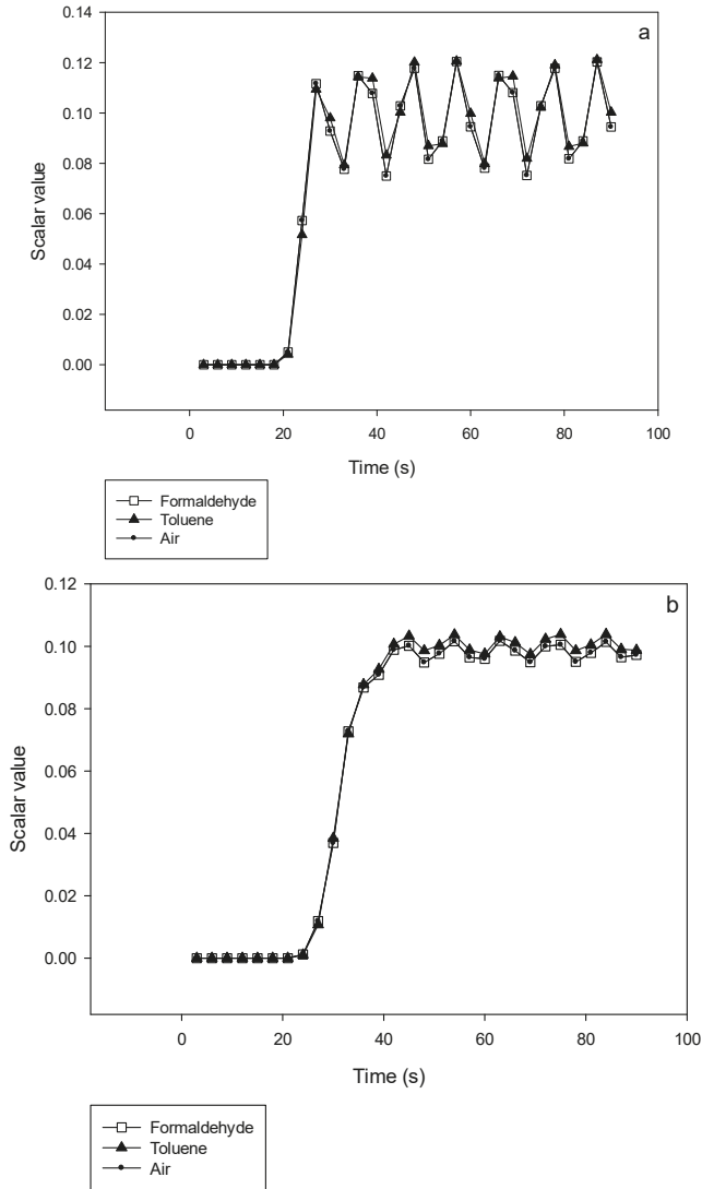
Figure 8. Comparison of the mixing's efficiency between formaldehyde, toluene and air being mixed with pure air at 25 \text{ NmL}\cdot\text{min}^{-1} . Variations of the scalar value with time at the exit of a 2-stages (a) or 4-stages (b) device, illustrating that there is almost no time response difference between formaldehyde, toluene and air.
