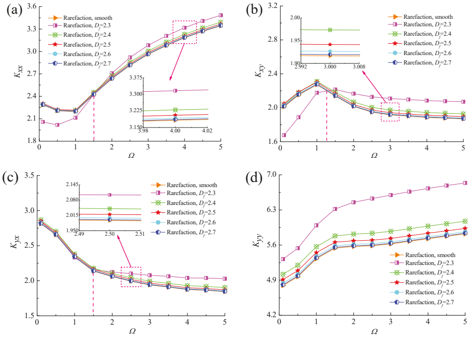
Figure 12. Effect of perturbation frequency on dynamic stiffness coefficients with different fractal dimensions. (a) K_{xx} vs. \Omega ; (b) K_{xy} vs. \Omega ; (c) K_{yx} vs. \Omega ; (d) K_{yy} vs. \Omega .
