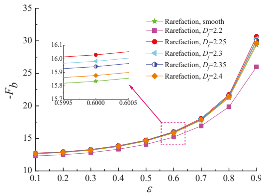
Figure 8. Static friction coefficient versus eccentricity ratio for different fractal dimensions at \Lambda = 20, G = 1 \times 10^{-11} .
