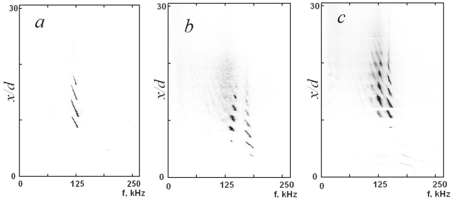
Figure 12. Spectra of acoustic oscillations generated by the underexpanded air jet in the plane of the normalized distance from the nozzle versus frequency for n = 1.75 (a), 2.5 (b), and 3 (c) for d = 0.72 mm and D = 0.4 mm.
