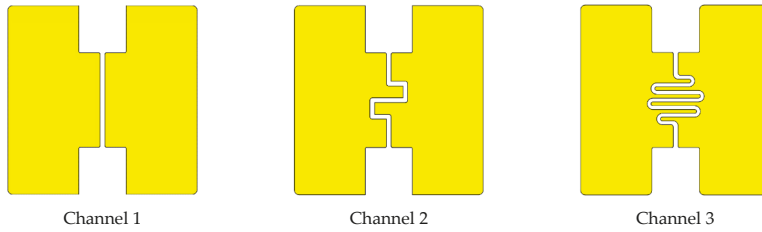
Figure 3. Microchannels for ionization chamber.
