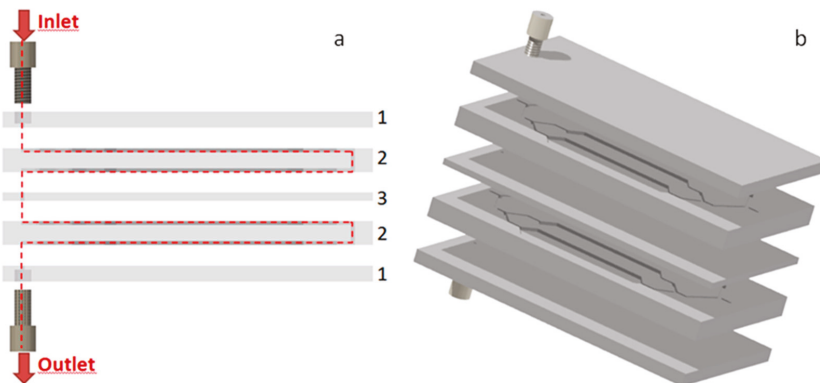
Figure 4. (a) Principle of the multi-stage design. The red line displays the path of the fluid flow. The design is made of 3 different chips: 1. This chip is used to fix a 1/16'' outer diameter connector serving as inlet or outlet ports. It is also the rooftop for microchannels; 2. The chip presents 2 patterns containing 4 buffer zones each, one on each side of the chip. The outlet of one pattern is connected to the inlet of the other via a hole. 3. An intermediate chip used as a rooftop for microchannels, separates the channels of the different chips number 2. (b) 3D schematics of the 4-stage mixer.
