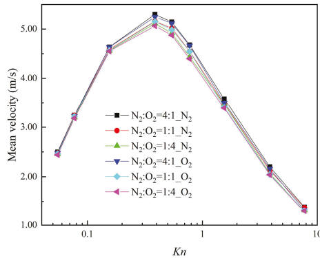
Figure 7. Mean velocities for different Knudsen numbers.
