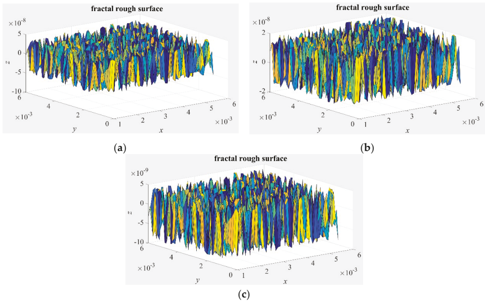
Figure 1. Simulation of a three-dimensional fractal surface topography for different fractal dimensions. (a) D_f = 2.2 , and G = 1 \times 10^{-10} m; (b) D_f = 2.3 , and G = 1 \times 10^{-10} m; (c) D_f = 2.4 , and G = 1 \times 10^{-10} m.
