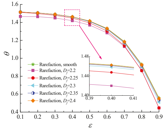
Figure 7. Attitude angle versus eccentricity ratio for different fractal dimensions at \Lambda = 20, G = 1 \times 10^{-11} .
