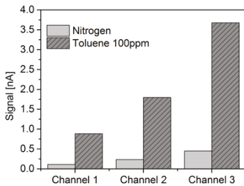
Figure 9. Signal for Channels 1, 2 and 3 using nitrogen and toluene 100 ppm as gas samples. Flow rate 20 mL/min and 30 V on electrodes. Relative uncertainty for signals of Channel 1 with nitrogen and toluene 100 ppm are 1.9% and 0.3%. Relative uncertainty for signals of Channel 2 with nitrogen and toluene 100 ppm are 0.8% and 0.2% respectively. Relative uncertainty for signals of Channel 3 with nitrogen and toluene 100 ppm are both 0.4%.
