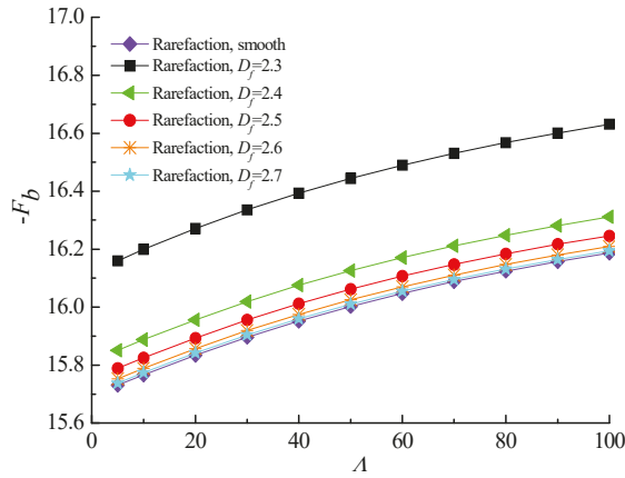
Figure 11. Static friction coefficient versus bearing number for different fractal dimensions at \varepsilon = 0.6 , G = 1 \times 10^{-10} .
