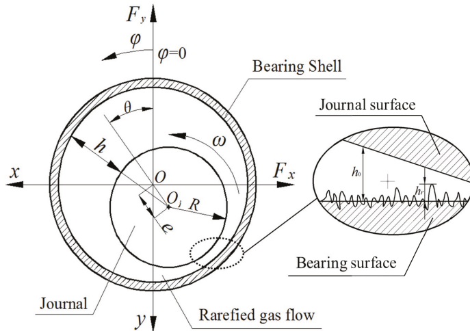
Figure 3. Geometrical configuration of the micro gas-lubricated journal bearing with rough surface.
