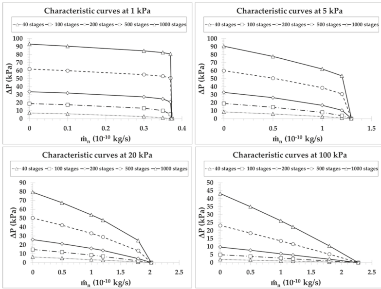
Figure 10. Performance characteristic curves of a Knudsen pump, based on pump C, for a number of stages N = 40, 100, 200, 500, 1000 with inlet pressures P_{in} = 1, 5, 20, 100 kPa when narrow microchannels diameter d = 10 \mu\text{m} and wide channel diameter D = 100 \mu\text{m} .
