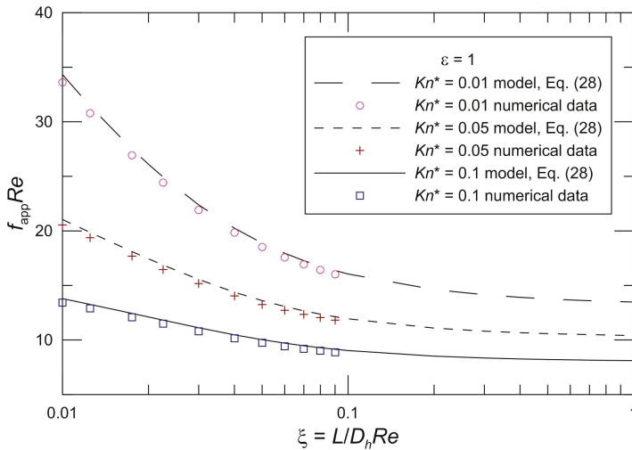
Figure 6. Comparison of f_{app}Re for our numerical data.
