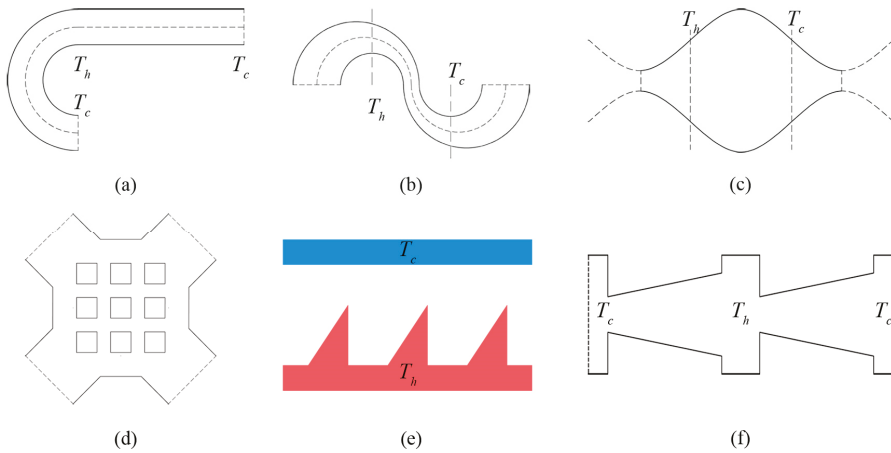
Figure 1. Common Knudsen pump channel structures: (a) Curve-straight channel, (b) double-curves channel, (c) sinusoidal channel, (d) matrix channel, (e) ratchet channel, (f) taper channel.
