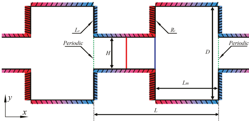
Figure 2. Configuration and geometric parameters.
