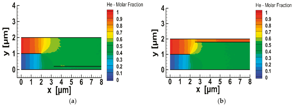
Figure 7. Gas mixing of He-Xe in the micro-mixer with splitter: Molar fraction contours of He with the splitter positioned at points (a) (3.25, 0.2) and (b) (2.5, 1.8).
