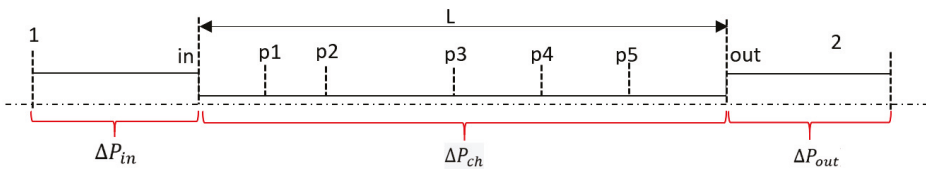
Figure 3. Schematic of minor losses.
