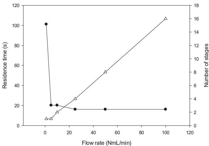
Figure 7. Number of stages ( \Delta ) required for the oscillations of the scalar value at the micromixer's exit to be lower than 5% of the targeted value 0.1 at flow rates ranging from 1 to 100 NmL·min -1 . Variations of the residence time ( \bullet ) with the flow rate for the corresponding number of stages required. At 100 NmL·min -1 , the 5% threshold is not reached: the percentage of oscillations is 6.1% after the 16th stage of mixing.
