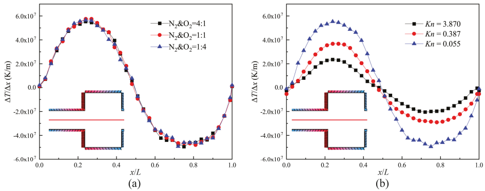
Figure 6. Temperature gradient on the central axis of the channel. (a) Kn = 0.055 ; (b) N_2 and O_2 = 4:1 .
