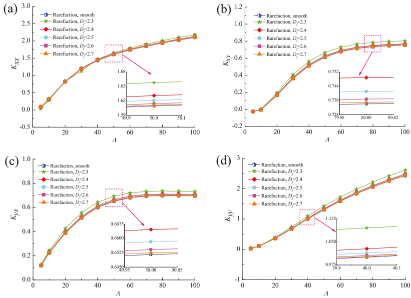
Figure 16. Effect of bearing number on dynamic stiffness coefficients with different fractal dimensions. (a) K_{xx} vs. \Lambda ; (b) K_{xy} vs. \Lambda ; (c) K_{yx} vs. \Lambda ; (d) K_{yy} vs. \Lambda .
