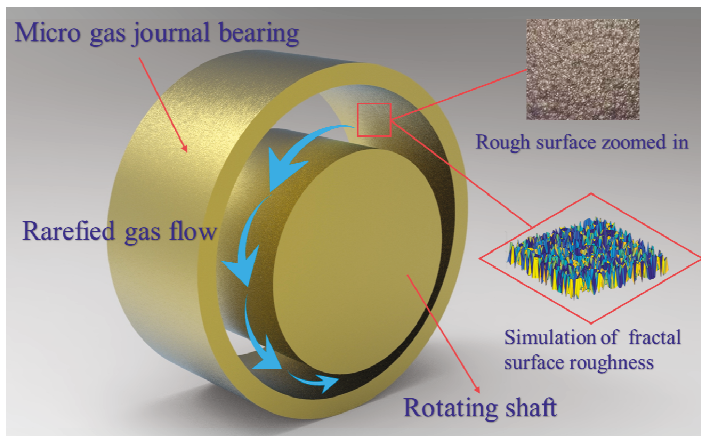
Figure 2. Schematic of a rough-surface gas-lubricated journal microbearings.
