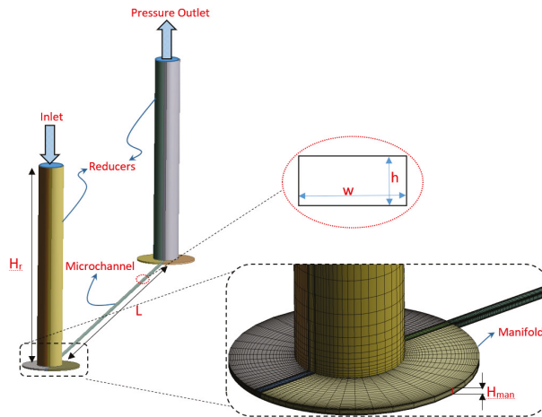
Figure 4. Details of numerical model and meshing.
