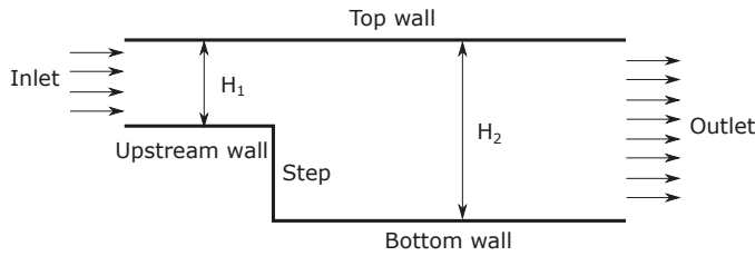
Figure 2. Schematic of backward-facing step.
