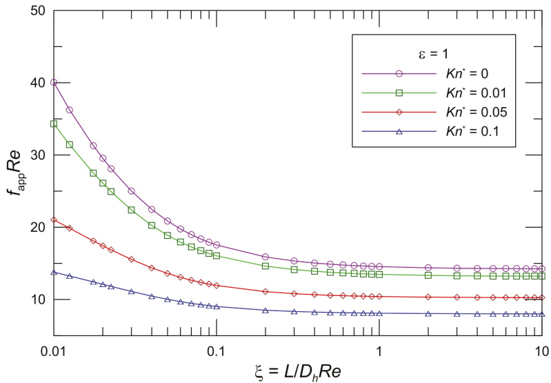
Figure 4. Effect of Kn^* on f_{app} Re for rectangular ducts ( \epsilon = 1 ).
