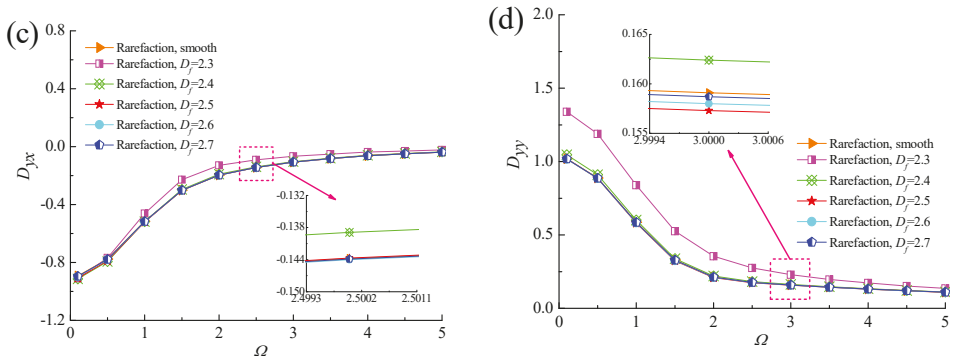
Figure 13. Effect of perturbation frequency on dynamic damping coefficients with different fractal dimensions. (a) D_{xx} vs. \Omega ; (b) D_{xy} vs. \Omega ; (c) D_{yx} vs. \Omega ; (d) D_{yy} vs. \Omega .
