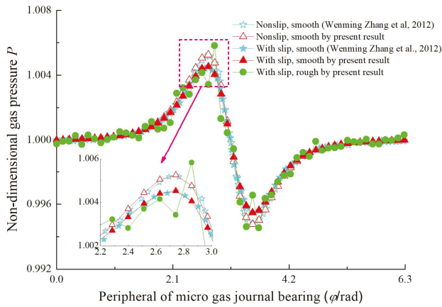
Figure 4. Comparison of dimensionless gas film pressure with Zhang et al. [20].
