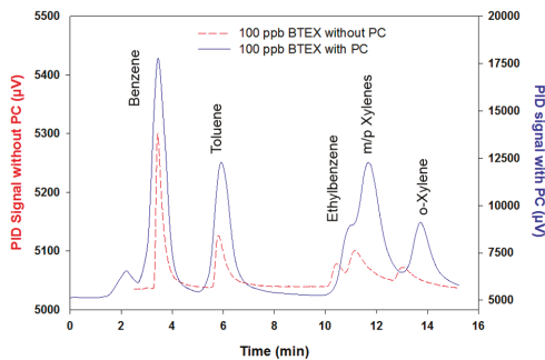
Figure 8. Red dashed line: Chromatogram of 100 ppb BTEX without pre-concentration step (sample volume of 200 \mu L). Blue solid line: Chromatogram of 100 ppb BTEX with pre-concentration step (sample volume of 20 mL).
