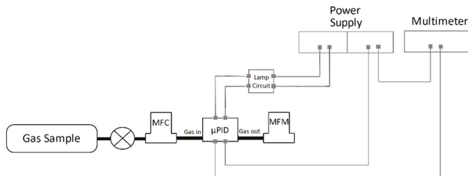
Figure 6. Experimental setup used for signal measurements from μPID prototype.
