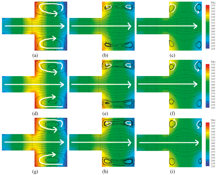
Figure 5. Velocity streamlines and temperature contours for different ratios of N_2 and O_2 and different Knudsen numbers. (a) N_2 and O_2 = 4:1 , Kn = 0.055 ; (b) N_2 and O_2 = 4:1 , Kn = 0.387 ; (c) N_2 and O_2 = 4:1 , Kn = 3.87 ; (d) N_2 and O_2 = 1:1 , Kn = 0.055 ; (e) N_2 and O_2 = 1:1 , Kn = 0.387 ; (f) N_2 and O_2 = 1:1 , Kn = 3.87 ; (g) N_2 and O_2 = 1:4 , Kn = 0.055 ; (h) N_2 and O_2 = 1:4 , Kn = 0.387 ; (i) N_2 and O_2 = 1:4 , Kn = 3.87 .
