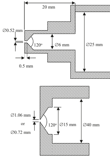
Figure 1. Nozzle scheme.
