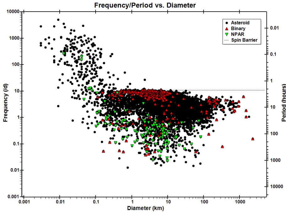
Fig. 1 Spin period for more than 5500 asteroids as function of their estimated diameter. A ‘spin barrier,’ above which no large objects will rotate, is apparent; consistent with a gravitational aggregate structure of loose conglomerations held together by mutual gravitation. Conversely, small objects can spin very fast, with full rotation within minutes; a hint towards a more monolithic structure. Near Earth objects are predominant in the population of objects smaller than approximately 1 km. (Source: the LCBD light curve database (Warner et al 2009)).
