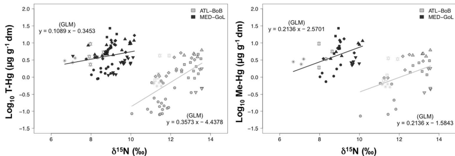
Figure 4. Relationships between individual log-transformed total Hg (T-Hg) concentrations (left panel, N = 134 ) or methyl-Hg (Me-Hg) concentrations (right panel, n = 75 ), and \delta^{15}\text{N} values (as a proxy of the trophic level within a given systems), for the seven species analysed in the NW Mediterranean - Gulf of Lion (MED - GoL) and in the NE Atlantic - Bay of Biscay (ATL - BoB). The symbology used for each species is the same as in Fig. 2c. Results from the GLMs (lines) are plotted on observed log-transformed data. When the interaction term was not significant (i.e. for MeHg, the model assumes that the form of the relationship is not different between the ecosystems), lines are parallel (i.e. same slope, although different intercept). This can also be interpreted (i.e. slope of the lines) as the biomagnification power of T-Hg or Me-Hg within each ecosystem considered (as performed by Cossa et al., 2012; for Me-Hg). Finally, the equations of lines (derived from model outputs; Table 2) are indicated.
