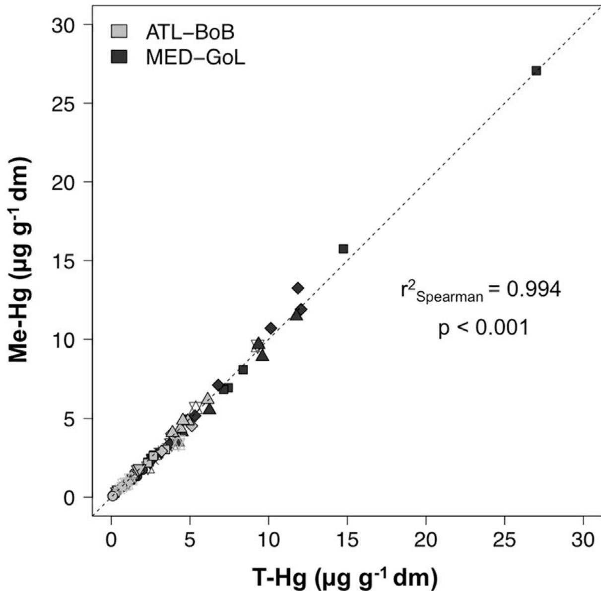
Figure 3. Relationship between muscle methyl-Hg (Me-Hg) and total Hg (T-Hg) concentrations for the subsample of individuals analysed for Me-Hg concentrations ( n = 75 ), and for the seven species analysed in the NW Mediterranean e Gulf of Lion (MED - GoL) and in the NE Atlantic e Bay of Biscay (ATL - BoB). The correspondence line 1:1 is indicated, as well as the results of the non-parametric Spearman correlation coefficient test. Symbols used for species are the same than in Fig. 2c.
