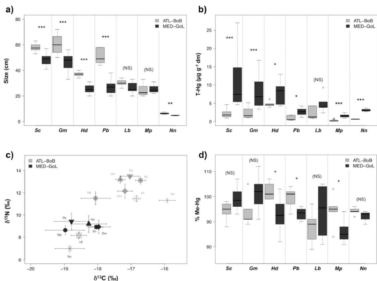
Figure 2. a) Boxplots of sizes (total length for fish, cephalothorax length for crustaceans) for the seven species analysed in the NW Mediterranean e Gulf of Lion (MED - GoL) and in the NE Atlantic -Bay of Biscay (ATL - BoB) (N = 134); b) Boxplots of muscle total Hg (T-Hg) concentrations (N = 134); c) Biplot of \delta^{13}\text{C} and \delta^{15}\text{N} values (N = 134); d) Boxplots of percentages of Me-Hg (i.e. ratios Me-Hg/T-Hg, in %) in the muscle of the subsample of individuals analysed for Me-Hg concentrations (n = 75). For boxplots (a, b, d), the box length represents the interquartile, the bar length represents the range, and the horizontal lines in bold are median values. For each species, the significant difference between systems is indicated (tested by Student t-test or Mann-Whitney-Wilcoxon test, depending on data satisfying conditions for parametric statistics or not). * p < 0.05 ; ** p < 0.01 ; *** p < 0.001 ; NS = non significant. For the biplot (c), values are mean \pm standard deviation per species. Abbreviations for species are specified in Table 1.
