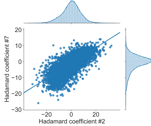
Fig. 2. Measurement scatter plot for two coefficients of the measurement vector. Each dot represents an image from the STL10 test set. The two histograms represents the marginal distribution of each variable while the full line on top of the scatter plot indicates the correlation between the two variables.
