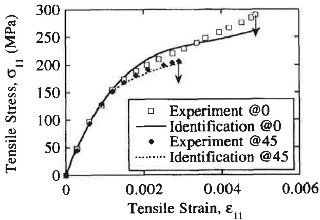
Fig. 1. Tension tests on a [0,90] SiC/SiC composite at 0° and 45°.
