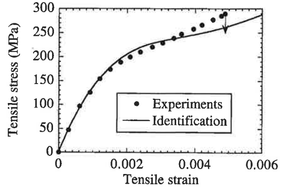
Fig. 3. Stress-strain curve at 0° for a SiC/SiC composite.
