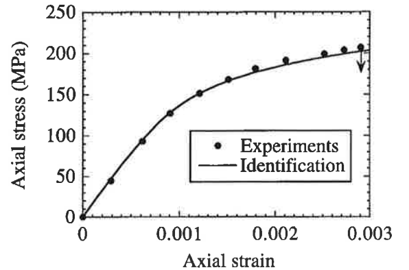
Fig. 4. Stress-strain curve at 45° for a SiC/SiC composite.
