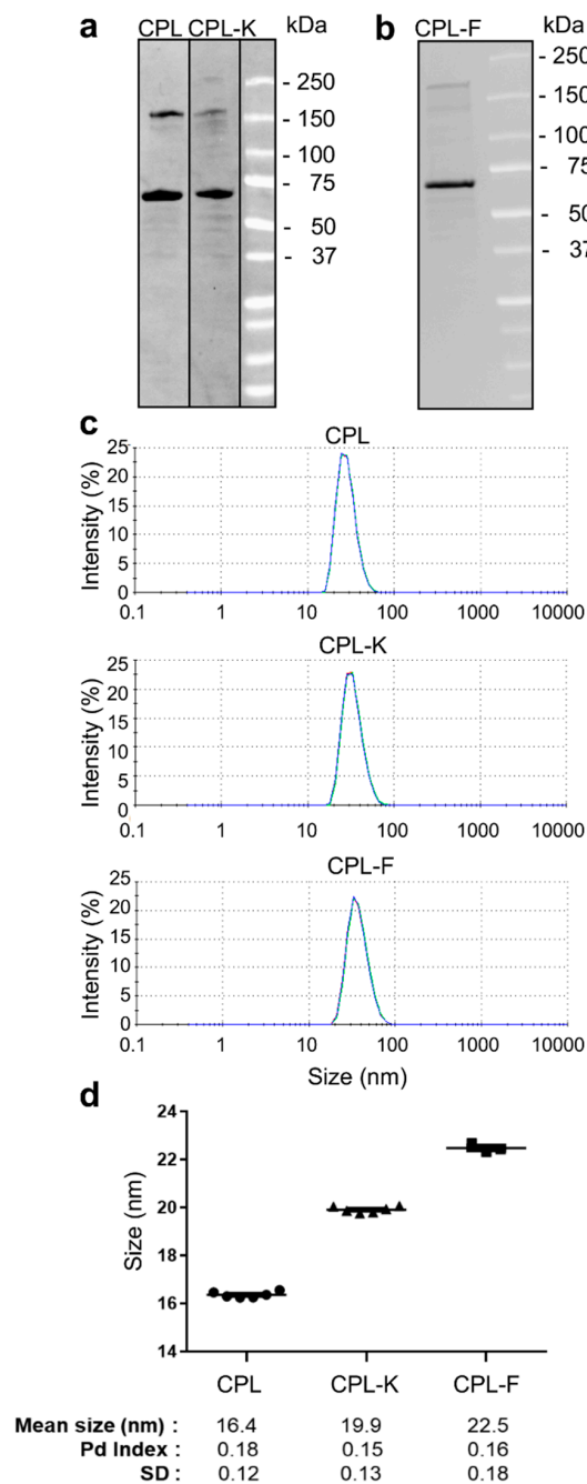
Figure 1. Analysis of CPL, CPL-K and CPL-F. (a,b) SDS-Page analysis of CPL, CPL-K (a) , and CPL-F (b) . The respective molecules are in the range of the estimated sizes of 59 kDa (CPL), 61 kDa (CPL-K) and 62 kDa (CPL-F). (c) Dynamic light-scattering (DLS) measurement of CPL, CPL-K and CPL-F. Measurements were performed three times independently for each of six samples per construct. (d) Mean particle sizes detected by DLS in the six samples per construct. Pd, polydispersion; SD, standard deviation.
