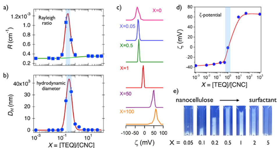
Figure 5: a) Rayleigh ratio \mathcal{R}(X) and b) hydrodynamic diameter D_H(X) for mixed cellulose nanocrystal/surfactant dispersions as a function of the mixing ratio X . Temperature is 25 \text{ }^\circ\text{C} and concentration c = 0.01 \text{ wt.}\% . In a), the continuous line in green is calculated for non-interacting species. The continuous lines in red are guides to the eyes. c) Intensity distributions as a function of the zeta potential \zeta for samples between X = 0 and X = 100 showing a displacement of the peak from negative (pure nanocrystalline cellulose) to positive (pure TEQ vesicles) zeta values. d) Zeta potential results \zeta(X) corresponding to the samples in c). The continuous line in red is a guide to the eyes. e) Images of mixed dispersions at c = 0.1 \text{ wt.}\% .
