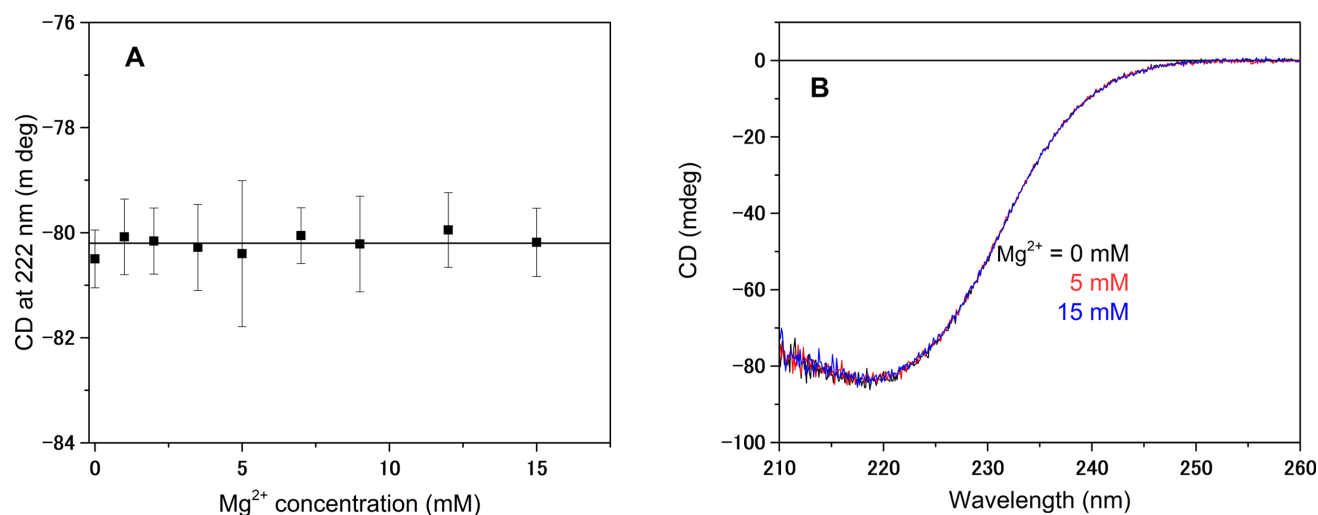
Figure 3. Mg 2+ ion causes no change in the CD signal of RecA. (A) CD signal intensity at 222 nm of 2 μM RecA, plotted as a function of Mg 2+ concentration. (B) CD spectra of 2 μM RecA in the presence of 0 mM (black), 5 mM (red) and 15 mM (blue) Mg 2+ are shown. All curves are superimposed and not distinguishable.
