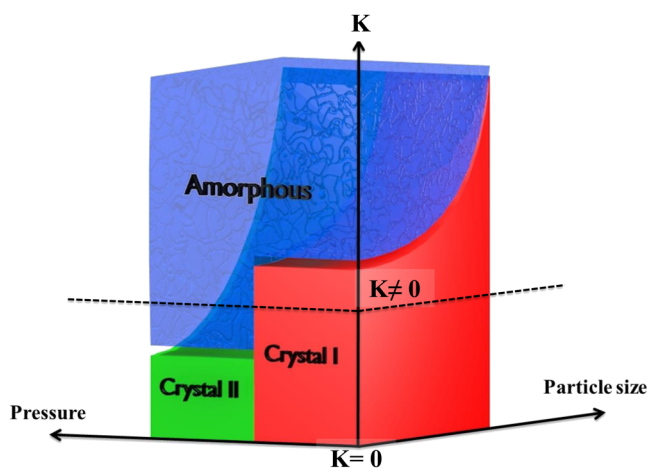
FIG. 3. Multidimensional plot (pressure, particle size, K ). The K factor corresponds to the Ginzburg term illustrating the effect of inhomogeneities such as defects, interface, and pressure gradient.
