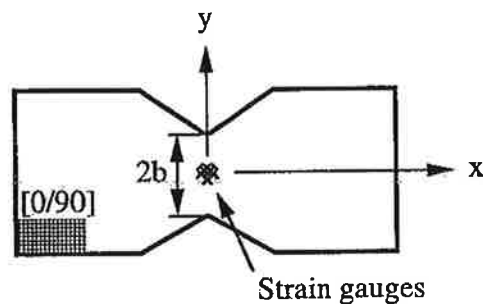
Fig. 9. – Iosipescu specimen configuration.
