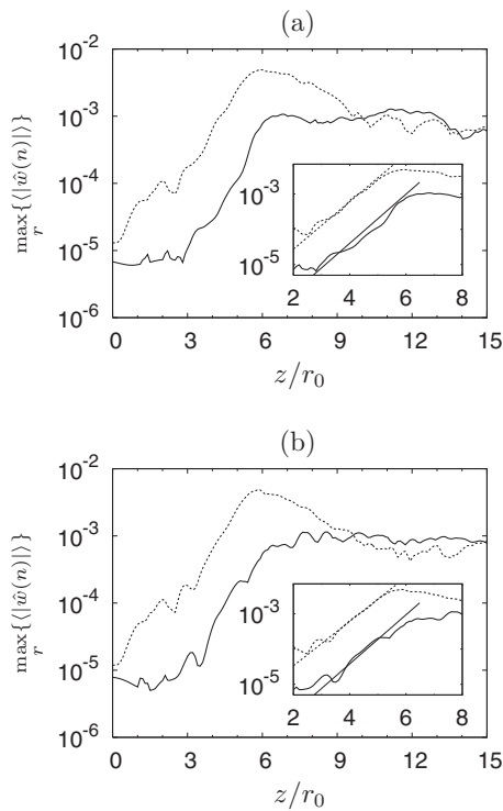
FIG. 17. Downstream development of Fourier modal amplitude \hat{w}(n) of azimuthal wavenumbers (—) n=0 and ( \cdots ) n=1 for (a) St_0^{n=0}=0.676 and (b) St_0^{n=1}=0.681 . Inlay shows zoomed axial region 2 \leq z/r_0 \leq 8 together with straight lines denoting growth rates according to linear stability theory.
