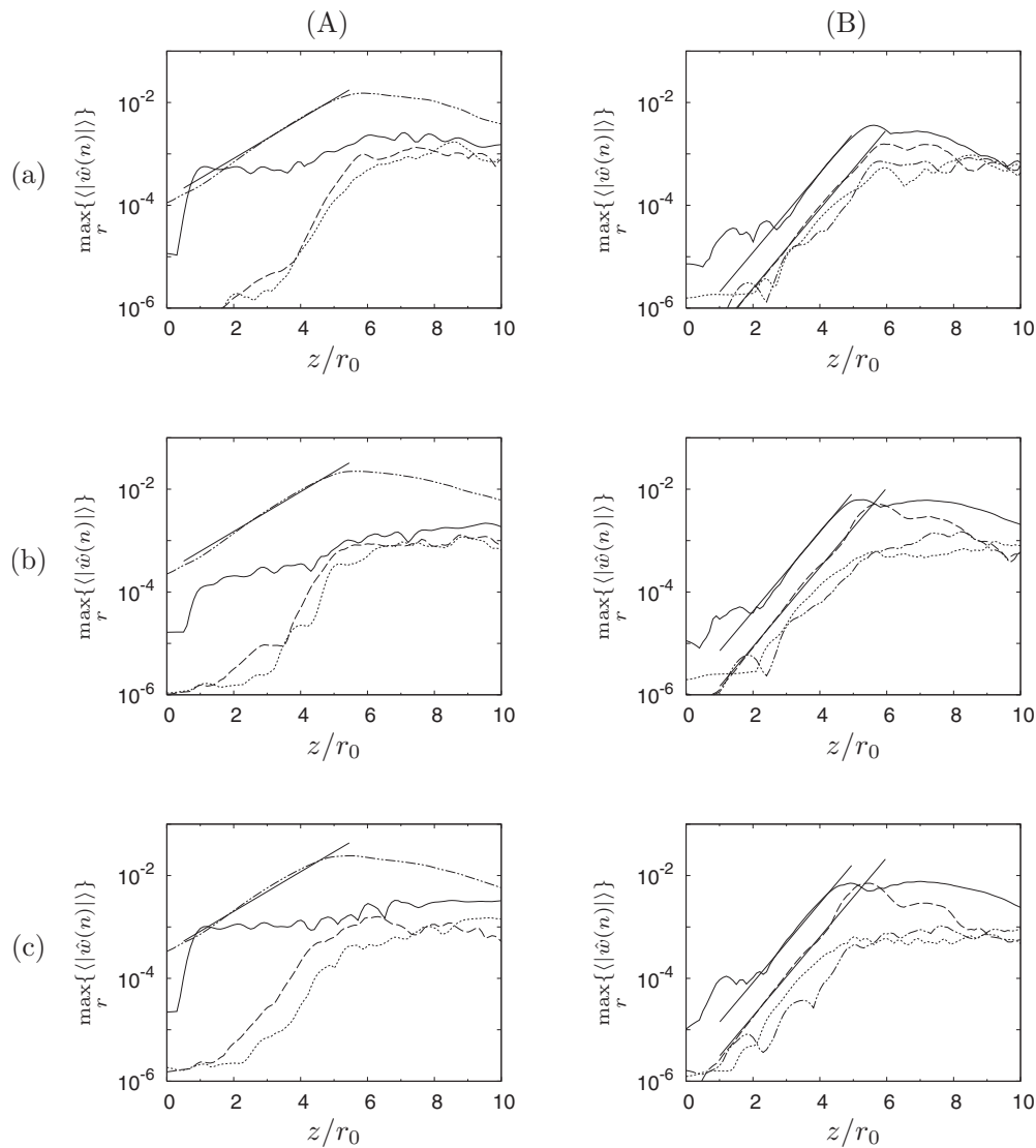
FIG. 20. Downstream development of Fourier mode amplitude \hat{w}(n) of azimuthal wavenumbers (—) n=0 , ( \cdots ) n=1 , ( -\cdots- ) n=4 , and ( --- ) n=8 : (a) Low, (b) Med, and (c) High for (A) fundamental frequency St_0^p and (B) peak frequency corresponding to higher harmonic St_1^p . Growth rates denoted by straight lines in row (A) according to linear theory and in row (B) according to weakly nonlinear theory.
