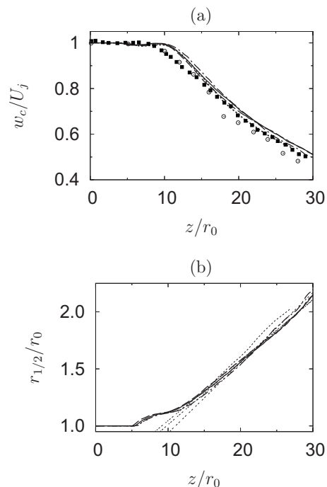
FIG. 9. (a) Mean axial velocity along the jet centerline w_c and (b) jet half width r_{1/2} : (\dots) Low , (\text{---}) Med , (\text{---}) High , (\dots) Bogey and Bailly (Ref. 16), (\circ) Lau et al. (Ref. 38), (\blacksquare) Arakeri et al. (Ref. 39); (\text{---}) , (\text{---}) , (\text{---}) denote the linear fit to the half-width development for cases Low , Med , and High .
