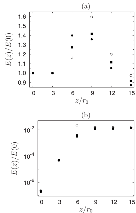
FIG. 11. One-dimensional turbulent kinetic energy of (a) varicose mode n=0 in linear scales and (b) first helical mode n=1 in logarithmic scales determined along the nozzle lip line at streamwise positions z/r_0 = i \times 3 ( i=0, \dots, 5 ) normalized by the kinetic energy of case Med at z=0 : E(n=0, z=0) = 3.73 \times 10^2 U_j^2 . (○) Low, (■) Med, and (●) High.
