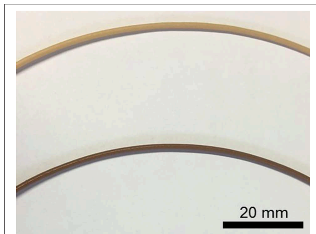
FIGURE 4 | Photographs of the wood flour (top) and rice husk (bottom) FDM filaments.
