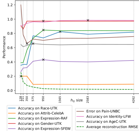
Figure 2. Impact of the size of h_G on the reconstruction error of \tilde{\mathcal{G}} and on the transfer for some of the target knowledge. Black cross is the optimal representation size for a given knowledge.
