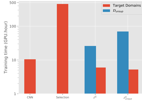
Figure 3. Total training time in hours (logscale) with one P100 GPU for different methods, on \mathcal{D}_{unsup} and on all target domains.
