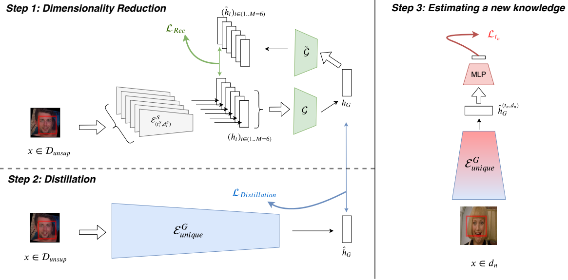
Figure 1. Overview of the method. Step 1 is the training of \mathcal{G} on \mathcal{D}_{unsup} , to obtain an encoder \mathcal{E}^G of x in a compact embedding h_G , gathering all sources of knowledge (represented by the extracted h_j ). Step 2 aims at reducing the number of parameters used to get h_G by distilling the knowledge of 130 millions parameters into a much simpler encoder \mathcal{E}_{unique}^G , leading to \hat{h}_G . In step 3 this lightweight encoder \mathcal{E}_{unique}^G can then be plugged with a MLP \mathcal{C}_{(t_n, d_n)} and all parameters adapted to learn new knowledge \mathcal{K}_{(t_n, d_n)} .
