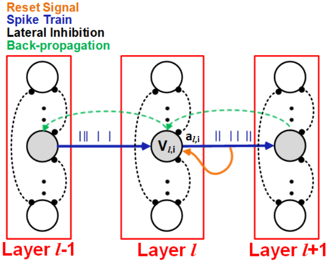
Fig. 2: Deep SNN equipped with backpropagation proposed by Lee et. al. [57]. The neuron’s activation value, a_{l,i} , is given by the neuron’s membrane potential. The differentiable activation function, which is calculated by the neuron’s excitatory input, lateral inhibition, and threshold, is used for developing backpropagation using the chain rule. The output activation value of the current layer (layer l ) is used as input for the next layer in the backpropagation algorithm.
