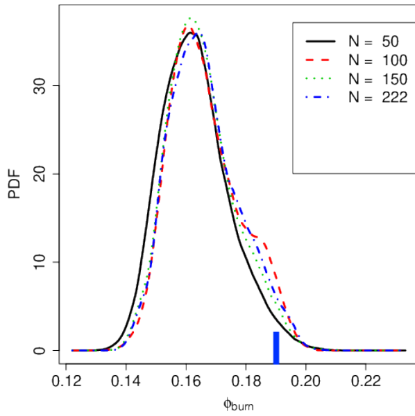
(a) Burned equivalence ratio, d/16 , \phi_{\text{burn}}
