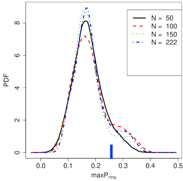
(c) Maximum RMS Pressure, d/16 , \max P_{\text{rms}}
