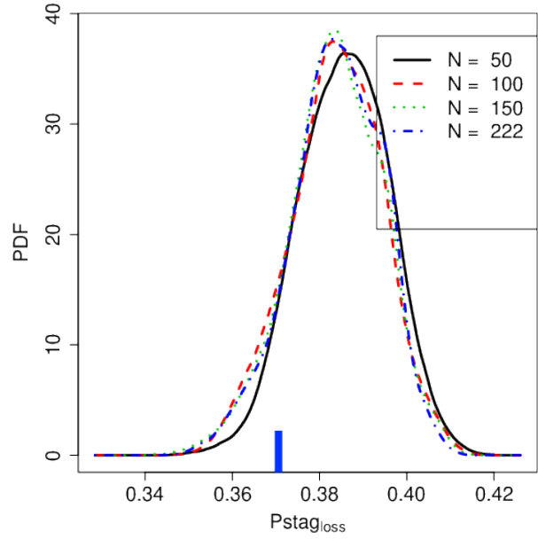
(b) Stagnation pressure Loss, d/16 , P_{\text{stagloss}}
