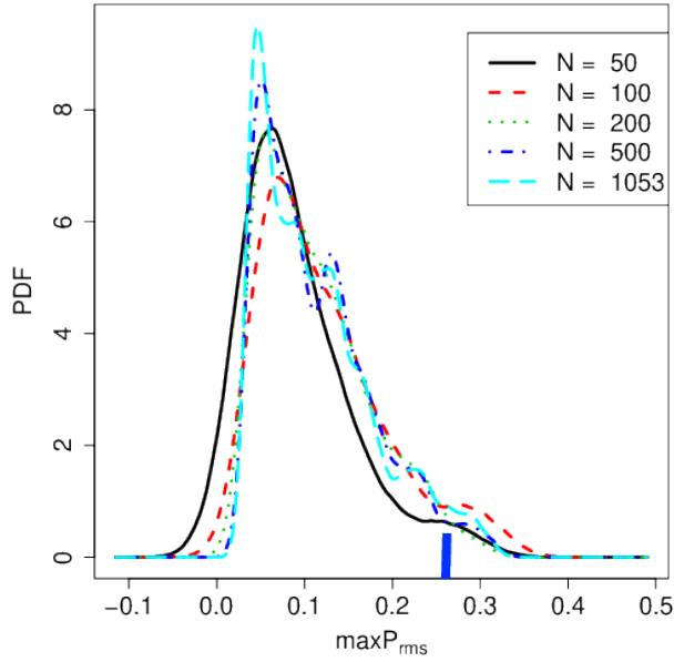
(c) Maximum RMS Pressure, d/8 , \max P_{\text{rms}}
