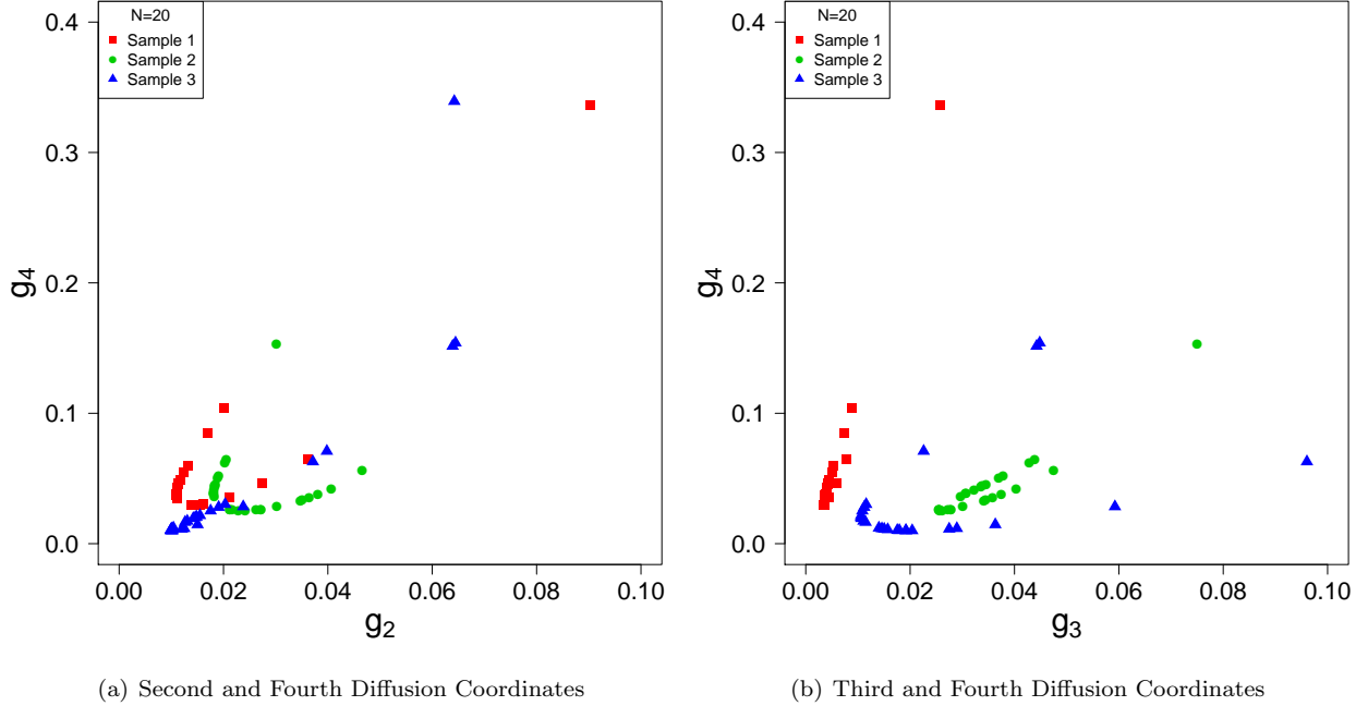
Figure 5: Scatter plot for second and fourth (a) and third and fourth (b) diffusion coordinates obtained for three samples each of size N=20 .
