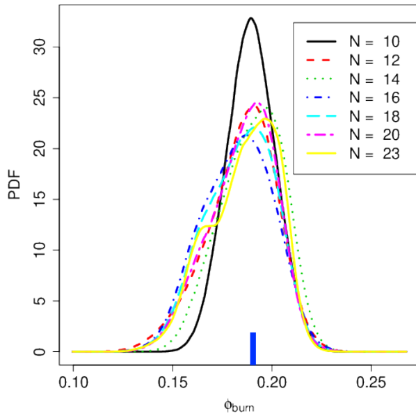
(a) Burned equivalence ratio, d/32 , \phi_{\text{burn}}
