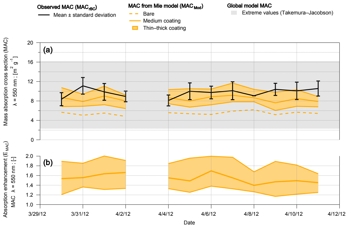
Figure 7. (a) Daily mean values of black carbon mass absorption cross section from observation ( \text{MAC}_{\text{rBC}} ) and from observationally constrained Mie calculations ( \text{MAC}_{\text{Mod}} ). Grey shadows represent the maximum and minimum MAC values used for radiative transfer simulations in global models (Jacobson, 2012; Takemura et al., 2000, 2002, 2005). (b) Daily mean values of absorption enhancement factor defined as the ratio of \text{MAC}_{\text{Mod}} for coated BC to that of bare BC. All values are for a wavelength of 550 nm.
