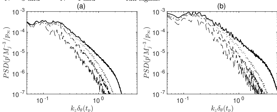
FIGURE 11. Pressure fluctuation spectra at r = 8r_0 at t = t_p + 12r_0/a_\infty for (a) M_j = 2 and (b) M_j = 3 ; partial sum of the azimuthal modes from mode 0 to mode N , with - - - N = 0 , - · - N = 1 , and ····· N = 4 and — full signal.
