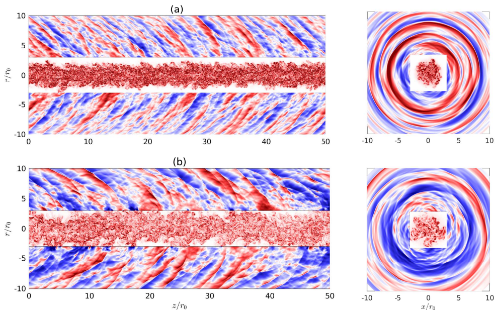
FIGURE 8. (Colour and movie available online at journals.cambridge.org/flm ) Snapshots of pressure fluctuations and vorticity norm at t = t_p + 12r_0/a_\infty for (a) M_j = 2 and (b) M_j = 3 . The colour scales range from -0.02p_\infty M_j^{3/2} to 0.02p_\infty M_j^{3/2} for the pressure and up to 3u_j/r_0 for the vorticity, from blue to red.
