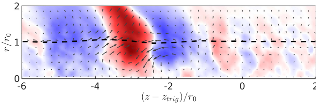
FIGURE 17. (Colour and movie available online at journals.cambridge.org/film ) Conditionally-averaged pressure and velocity at t = t_p + 2r_0/a_\infty for M_j = 2 . The pressure fluctuations are represented in colour, the arrows represent the velocity fluctuations and the dashed line indicates the sonic line. The colour scale for the pressure ranges from -0.1p_\infty to 0.1p_\infty , from blue to red.
