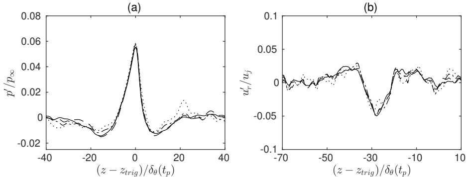
FIGURE 21. Representation for M_j = 2 of (a) the conditional pressure fluctuations at r = 8r_0 and t = t_{trig} and (b) the radial velocity fluctuations at r = 0.5r_0 and t = t_p + 2r_0/a_\infty , computed using — N_0 , - - - N_0/2 , - · - N_0/4 and · · · · N_0/8 events.
