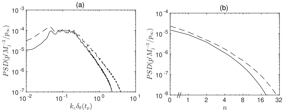
FIGURE 9. Pressure fluctuation spectra at t = t_p + 12r_0/a_\infty normalised by p_\infty M_j^3 as a function of (a) axial wavenumber and (b) azimuthal mode number for — M_j = 2 and - - - M_j = 3 .
