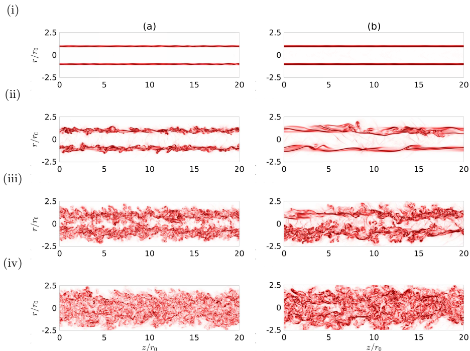
FIGURE 3. (Colour available at journals.cambridge.org/flm ) Vorticity norm for (a) M_j = 2 and (b) M_j = 3 at times (i) t = 5r_0/u_j , (ii) t_c - 10r_0/u_j , (iii) t_c and (iv) t_c + 10r_0/u_j . The colour scale ranges up from 0 to 5u_j/r_0 , from white to red.
