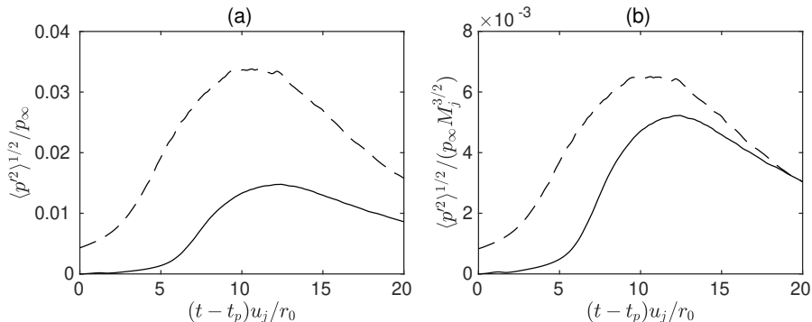
FIGURE 7. Time variations of the RMS value of pressure fluctuations at r = 8r_0 normalised by (a) p_\infty and (b) p_\infty M_j^{3/2} for — M_j = 2 and - - - M_j = 3 .
