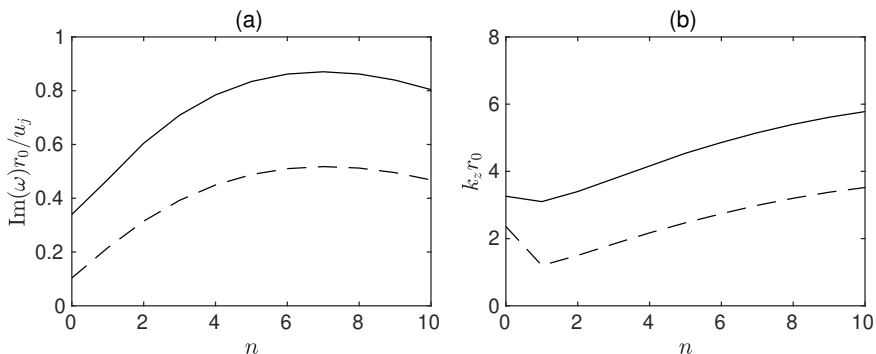
FIGURE 2. Representation of the (a) maximum amplification rate and (b) the most amplified axial wavenumber as a function of the azimuthal mode number for — M_j = 2 and - - - M_j = 3 .
