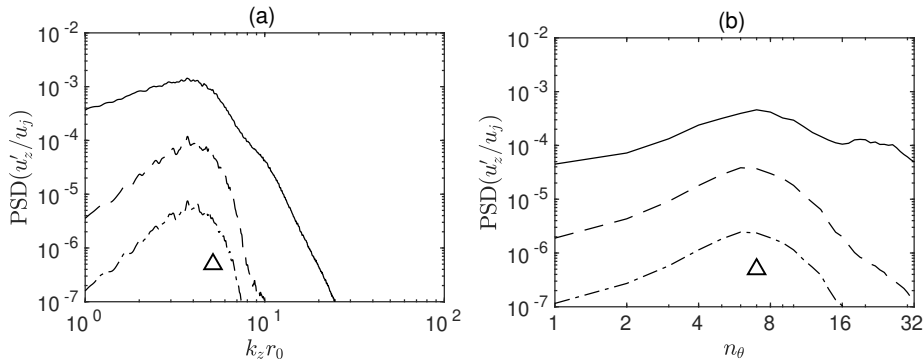
FIGURE 20. Power spectrum densities of the axial velocity fluctuations for the jet at M_j = 2 at r = r_0 and t = 5r_0/u_j as a function of (a) the axial wavenumber and (b) the azimuthal mode number, and for three values of the excitation strength parameter \alpha_{\text{exc}} : — \alpha_{\text{exc}} = 0.04 , - - - \alpha_{\text{exc}} = 0.01 and — · — \alpha_{\text{exc}} = 0.0025 . The triangles indicate the most amplified wavenumbers and mode numbers at t = 0 .
