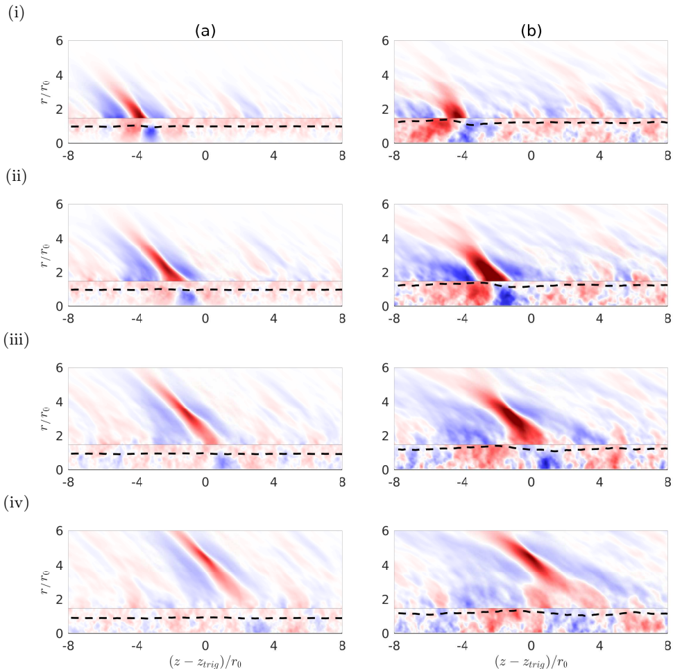
FIGURE 15. (Colour and movie available online at journals.cambridge.org/flm ) Conditionally-averaged pressure and radial velocity fluctuations for (a) M_j = 2 and (b) M_j = 3 at times (i) t_p + 1.5r_0/a_\infty , (ii) t_p + 3r_0/a_\infty , (iii) t_p + 4.5r_0/a_\infty and (iv) t_p + 6r_0/a_\infty . The dashed line indicates the sonic line and the colour scales range from -0.03p_\infty M_j^{3/2} to 0.03p_\infty M_j^{3/2} for the pressure and up to 0.1u_j for the radial velocity, from blue to red.
