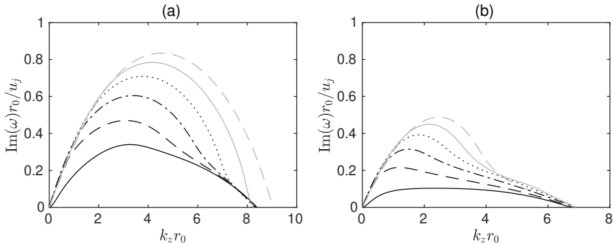
FIGURE 1. Amplification rates of the Kelvin-Helmholtz instability waves at t = 0 for (a) M_j = 2 and (b) M_j = 3 ; modes — n = 0 , - - - n = 1 , - · - n = 2 , ····· n = 3 , — n = 4 and - - - n = 5 .
