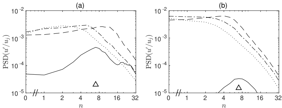
FIGURE 6. Representation, for (a) M_j = 2 and (b) M_j = 3 , of the power spectrum densities of axial velocity fluctuations at r = r_0 normalised by u_j as a function of the azimuthal mode number at times — 5r_0/u_j , - - - t_p , - · - t_p + 10r_0/u_j and ····· t_p + 20r_0/u_j . The triangle indicates the most amplified mode number at t = 0 .
