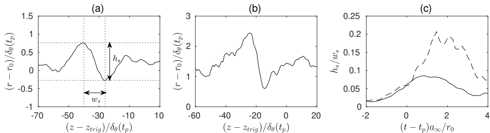
FIGURE 18. Radial position of the sonic line at t = t_p + 2r_0/a_\infty for (a) M_j = 2 and (b) M_j = 3 , and (c) time variations of the aspect ratio h_s/w_s of the sonic-line disturbance for — M_j = 2 and - - - M_j = 3 .
