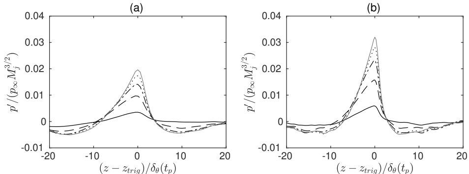
FIGURE 13. Axial profiles of the conditionally-averaged pressure in the plane \theta = \theta_{\text{trig}} at t = t_{\text{trig}} and r = r_{\text{trig}} for (a) M_j = 2 and (b) M_j = 3 ; partial sum up to order N with — N = 0 , - - - N = 1 , - · - N = 2 , · · · · · N = 3 , and — N = 4 .
