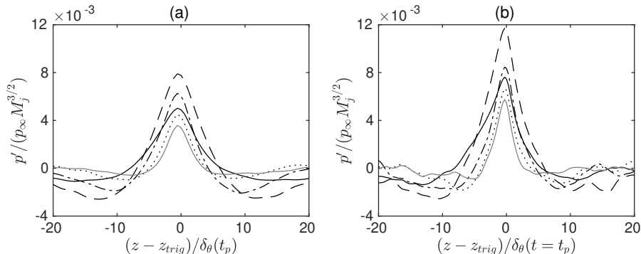
FIGURE 12. Axial profiles of the conditionally-averaged pressure at t = t_{\text{trig}} and r = r_{\text{trig}} for (a) M_j = 2 and (b) M_j = 3 ; azimuthal modes — n = 0 , - - - n = 1 , - · - n = 2 , ····· n = 3 , and — n = 4 .
