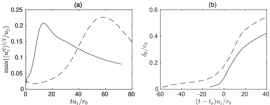
FIGURE 4. Time variations of (a) maximum RMS value of axial velocity fluctuations and (b) shear-layer momentum thickness for — M_j = 2 and - - - M_j = 3 .
