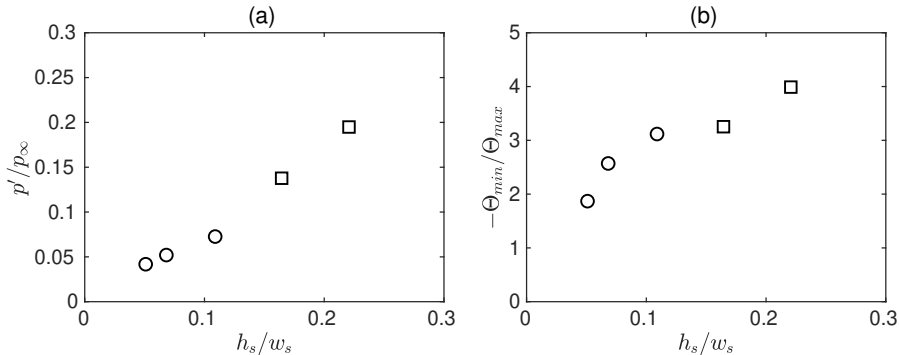
FIGURE 19. Representation of (a) the peak conditional pressure at r = r_{trig} and (b) the steepness parameter -\theta_{min}/\theta_{max} as a function of the aspect ratio of the sonic line disturbance at t = t_p + 2r_0/a_\infty for \circ M_j = 2 and \square M_j = 3 .
