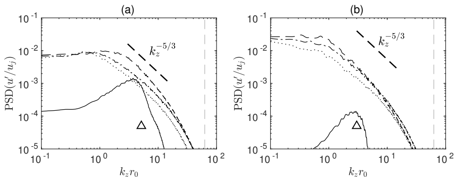
FIGURE 5. Representation, for (a) M_j = 2 and (b) M_j = 3 , of the power spectrum densities of axial velocity fluctuations at r = r_0 normalised by u_j as a function of the axial wavenumber at times — 5r_0/u_j , - - - t_p , - · - t_p + 10r_0/u_j and · · · · t_p + 20r_0/u_j . The triangle indicates the most amplified wavenumber at t = 0 and the dashed gray line indicates the grid cut-off wavenumber.
