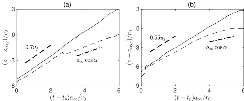
FIGURE 16. Time evolution of the axial positions of — minimum radial velocity and - - - maximum pressure in the plane at \theta = \theta_{\text{trig}} for (a) M_j = 2 and (b) M_j = 3 .
