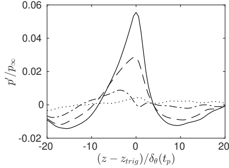
FIGURE 14. Conditionally-averaged pressure at r = r_{\text{trig}} and t = t_{\text{trig}} for M_j = 2 represented in the plane — \theta = \theta_{\text{trig}} , - - - \theta_{\text{trig}} + \pi/6 , - · - \theta_{\text{trig}} + \pi/3 , and · · · · \theta_{\text{trig}} + \pi/2 .
