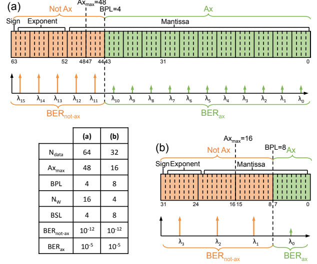
Figure 2: Example of floating point data approximation: a) IEEE 754-2008 double-precision (DP) format, b) IEEE 754-2008 single-precision (SP) format.
