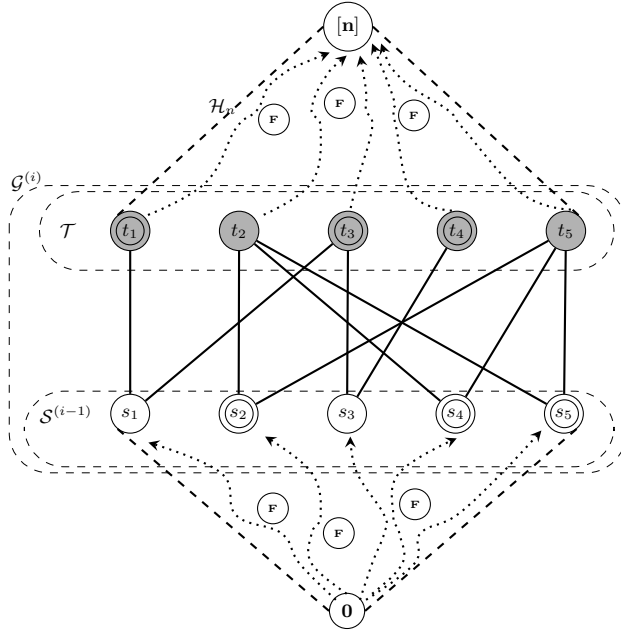
Fig. 5: The undirected bipartite graph \mathcal{G}^{(i)} = ((\mathcal{S}^{(i-1)}, \mathcal{T}), \subset) , and vertex cover \mathcal{X}^{(i)} = (X_S^{(i)}, X_T^{(i)}) (doubly-circular nodes).
