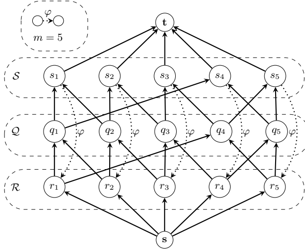
Fig. 1: The auxiliary network \mathcal{K} = (V_{\mathcal{K}}, A_{\mathcal{K}}) and bijection \varphi .
