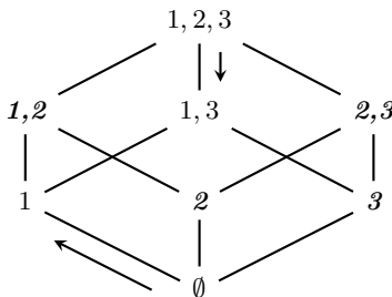
Fig. 3: A \text{double\_bfs\_phase}() on \mathcal{H}_3 that starts from S = \emptyset and T = \{1, 2, 3\} . The forbidden vertices are \mathcal{F} = \{\{2\}, \{3\}, \{1, 2\}, \{2, 3\}\} , while the edges explored by \text{BFS}_{\uparrow} and \text{BFS}_{\downarrow} are (\emptyset, \{1\}) and (\{1, 2, 3\}, \{1, 3\}) (respectively).
