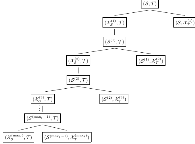
Fig. 4: The frontier sets of the compression_phase() .
