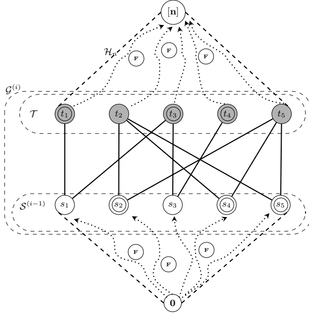
Fig. 5: The undirected bipartite graph \mathcal{G}^{(i)} = ((\mathcal{S}^{(i-1)}, \mathcal{T}), \subset) , and vertex cover \mathcal{X}^{(i)} = (X_{\mathcal{S}}^{(i)}, X_{\mathcal{T}}^{(i)}) (doubly-circular nodes).
