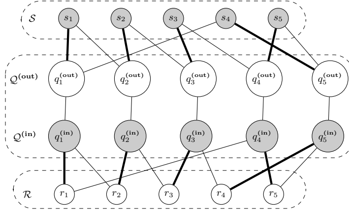
Fig. 2: The undirected bipartite graph \mathcal{K}' = (V_{\mathcal{K}'}, E_{\mathcal{K}'}) and a perfect matching \mathcal{M} (thick edges).
