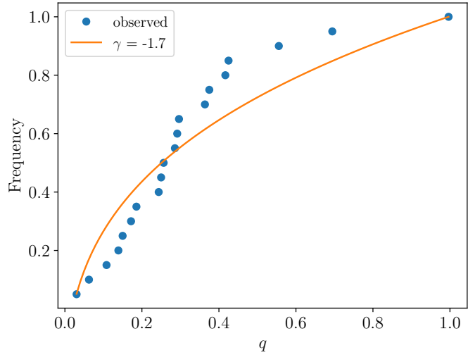
Fig. 20. Cumulative distribution of all mass ratios q and the best fit curve of a power law \propto q^\gamma = q^{-1.7 \pm 0.3} .
