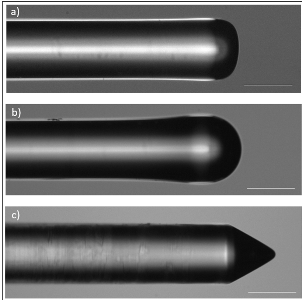
Fig. 1. Images of the three different fiber tips used for the experiments carried out. Scale bars corresponds to 100 \mu\text{m} . a) Fiber A with higher radius of curvature. b) Fiber B with intermediate radius of curvature. c) Fiber C with conical lensed tip.
