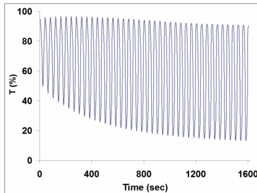
Figure 4. Evolution of the transmittance recorded at 630 nm during 40 CV cycles for NiO film deposited at J_d of -0.05 \text{ mA/cm}^2 .
