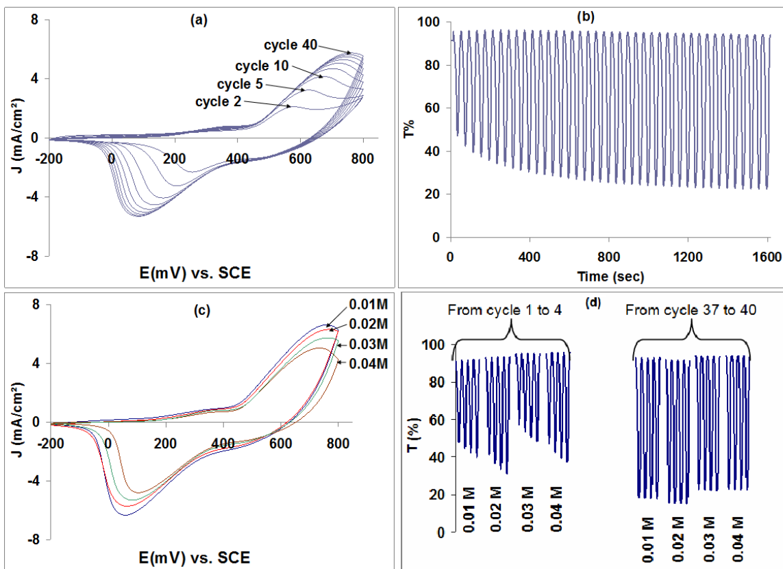
Figure 9. CV and transmittance spectra (recorded at 630 nm) for films deposited at different molar concentrations. (a) CV for film deposited at 0.04 M, (b) Transmittance during CV for films deposited at 0.04 M, (c) CV of cycle 40 for different deposited films, and (d) transmittance in activation and near saturation regions for different deposited films.
