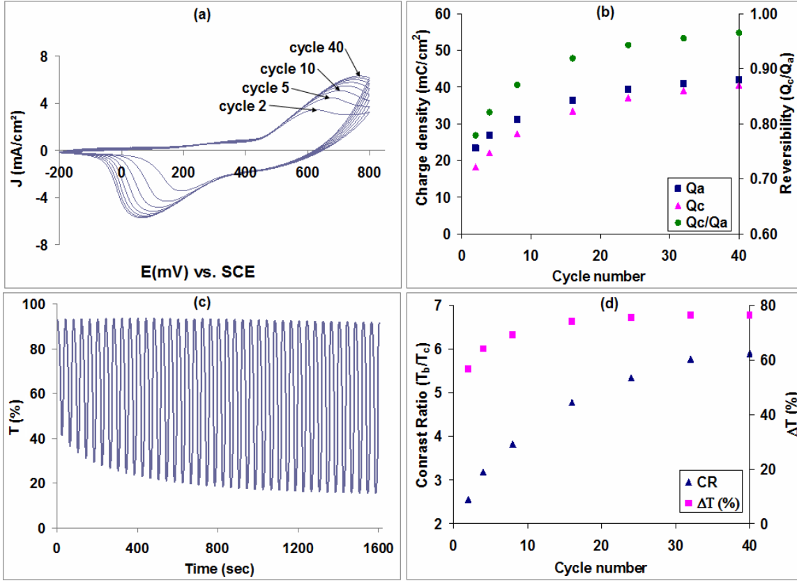
Figure 11. Electrochromic properties of optimized NiO film: a) 40 CV cycles, b) charge densities with corresponding reversibility, c) Transmittance during CV, and d) Transmittance modulation and corresponding contrast ratio.
