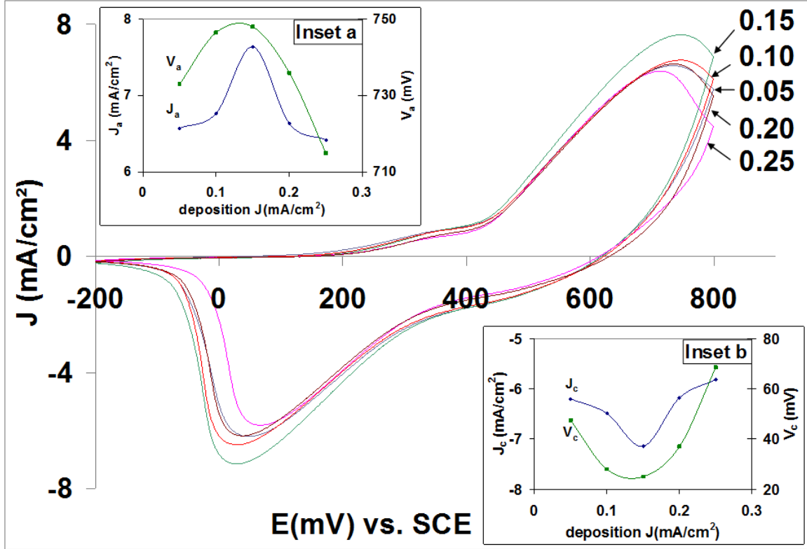
Figure 6. CVs for cycle 40 of films deposited at different J_d (-0.05, -0.10, -0.15, -0.20, and -0.25 mA/cm 2 ). Inset a is J_a and V_a and inset b is J_c and V_c variations for different deposited films.
