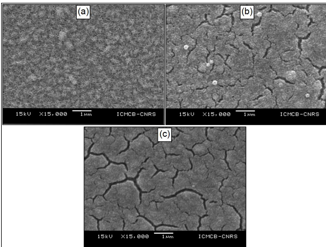
Figure 13. SEM images for NiO films deposited at (a) optimized parameters, (b) 0.01 M aqueous solution, and (c) -0.15 \text{ mA/cm}^2 current density.
