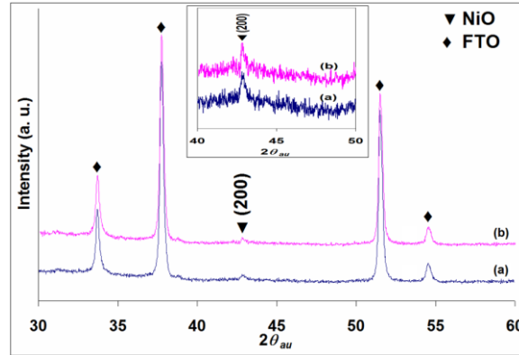
Figure 7. X-ray diffractogram of NiO thin films deposited at (a) -0.05 \text{ mA/cm}^2 and (b) -0.25 \text{ mA/cm}^2 on FTO/glass substrate. The inset shows a magnification of (200) peak.
