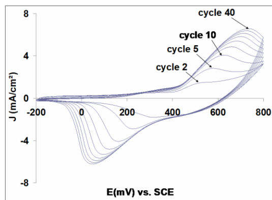
Figure 1. 40 cycles of CV for NiO films deposited at J_d = -0.05 \text{ mA/cm}^2 and cycled in a three electrodes cell, NiO/KOH (0.1 M)/Pt.
