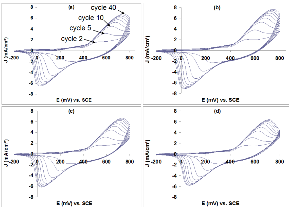
Figure 2. 40 CV cycles for NiO films deposited at different J_d of (a) -0.1 \text{ mA/cm}^2 , (b) -0.15 \text{ mA/cm}^2 , (c) -0.20 \text{ mA/cm}^2 and , (d) -0.25 \text{ mA/cm}^2 . All films are cycled in a three electrodes cell, NiO/KOH (0.1 M)/Pt.
