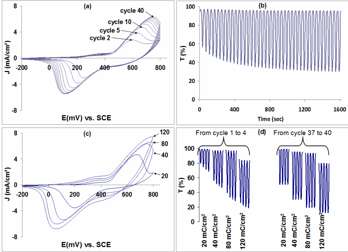
Figure 10. CV and transmittance spectra, recorded at 630 nm, for films deposited with different charge densities: (a) CV for film deposited with 40 mC/cm 2 , (b) Evolution of the transmittance during CV for films deposited with 40 mC/cm 2 , (c) CV of cycle 40 for films deposited with different Q_d (20, 40, 80, and 120 mC/cm 2 ), and (d) transmittance in activation and near saturation regions for films deposited with different Q_d .
