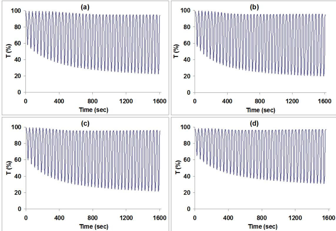
Figure 5. Evolution of the transmittance recorded at 630 nm during 40 CV cycles for NiO films deposited at J_d of (a) -0.1 \text{ mA/cm}^2 , (b) -0.15 \text{ mA/cm}^2 , (c) -0.20 \text{ mA/cm}^2 and , (d) -0.25 \text{ mA/cm}^2 .
