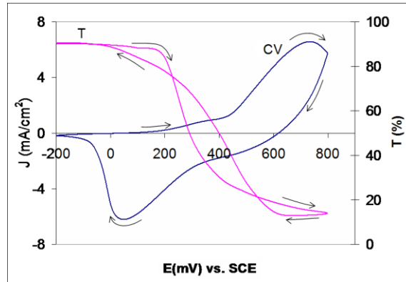
Figure 3. Variation of transmittance T at 630 nm during CV measurements for cycle number 40 of NiO film deposited at J_d of -0.05 \text{ mA/cm}^2 .
