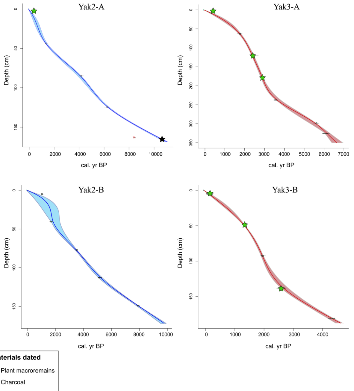
684 Figure 2: Age-depth model based on radiocarbon ages (see Table 2) from Yak2-A, Yak2-B, Yak3-A
