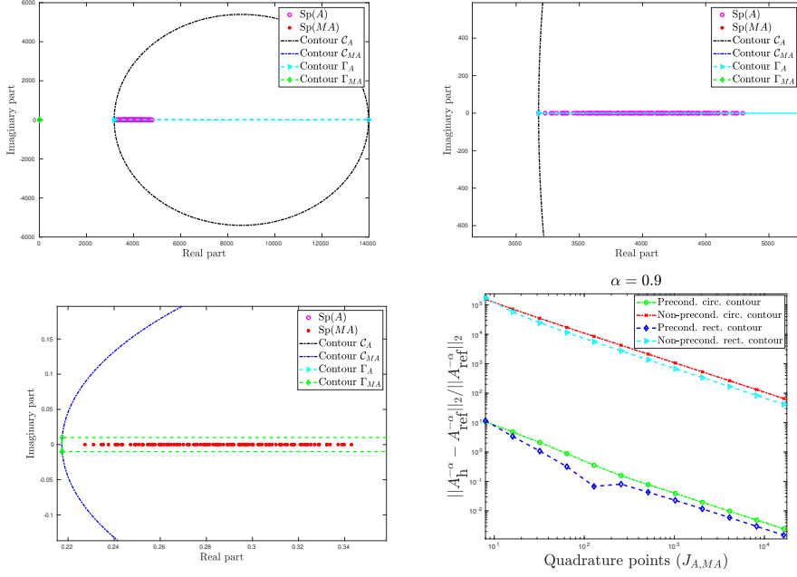
FIG. 4. Experiment 3. (Top-Left) Sp(A) and Sp(MA) , with A \in \mathbb{R}^{n \times n} , and C_A , C_{MA} , \Gamma_A , \Gamma_{MA} . (Top-Right) zoom on Sp(A) . (Bottom-Left) zoom on Sp(MA) . (Bottom-Right) Relative error vs the number of integration points for \alpha = 0.9 .
