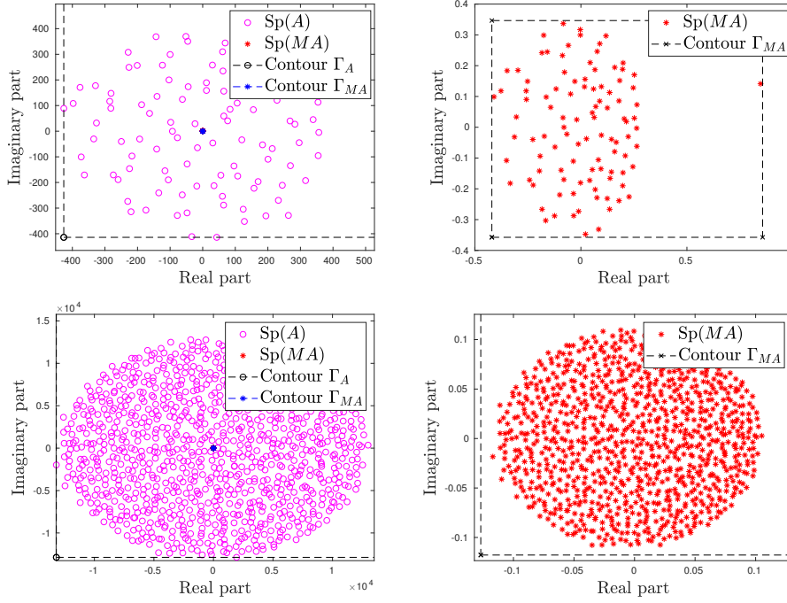
FIG. 3. Experiment 2. \text{Sp}(A) and \text{Sp}(MA) , and rectangular contour: (Top-Left) : n = 101 ; (Top-Right) : zoom for n = 101 ; (Bottom-Left) n = 1001 ; (Bottom-Right) : zoom for n = 1001 .
