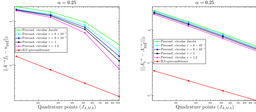
FIG. 12. Experiment 7. Jacobi preconditioner, differential-based preconditioner M_\tau with \tau = 8 \times 10^{-1} , \tau = 9 \times 10^{-1} , \tau = 1 , and \tau = 1.2 and ILU-preconditioner with a drop tolerance at 10^{-1} . (Left) In logscale \|A^{-\alpha} f_h - u_{\text{ref}}\|_2 where A^{-\alpha} f_h = u_h , as a function of the number of quadrature points J_{A,MA} , with \alpha = 0.25 , (Right) \|A_h^{-\alpha} - A_{\text{ref}}^{-\alpha}\|_2 in logscale as a function of the number of quadrature points J_{A,MA} , with n = 101 . (Right) Direct contour \mathcal{C}_A and preconditioned contour \mathcal{C}_{MA} .
