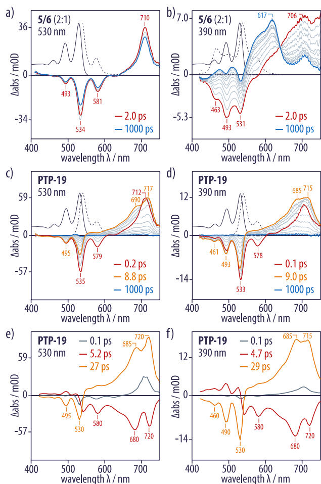
Figure 10. Transient absorption spectroscopy of the triad PTP-19 in solution revealed charge separation and recombination upon light absorption. a) TA spectra of the mixture 5/6 (2:1) excited at 530 nm showed the typical ground state bleaching, stimulated emission, and S_1 photoinduced absorption of the perylene bisimide without any influence of the quaterthiophene 6 . b) TA spectra of 5/6 (2:1) excited at 390 nm showed the quaterthiophene in the S_1 state, which evolved to the triplet state with a time constant of 400 ps, as well as an additional contribution from the perylene in the S_1 state since it is weakly absorbing at 390 nm; no influence of the perylene on the excited quaterthiophene was observed. c) TA spectra of PTP-19 excited at 530 nm: from the perylene in the S_1 state (red), charged species formed (orange), and recombined to the ground state (blue). d) TA spectra of PTP-19 excited at 390 nm were almost identical to c) , showing that an energy transfer from the quaterthiophene to the perylene occurred faster than the resolution of the experimental setup. e) Multi-exponential global analysis (Convolution of a Gaussian IRF with three exponential functions) of PTP-19 excited at 530 nm correlated charge separation to a time constant of 5 ps (red) and recombination to a time constant of 27 ps (orange). f) Multi-exponential global analysis of PTP-19 excited at 390 nm was almost identical to e) . Absorption and emission spectra of the samples are shown in solid and dashed black lines, respectively.
