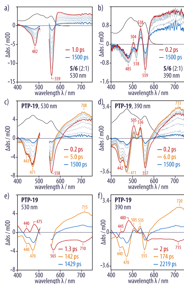
Figure 11. Transient absorption spectroscopy in thin films of PTP-19 showed a slower charge recombination than in solution and the formation of long-lived charge carriers. a) TA spectra of the mixture 5/6 (2:1) excited at 530 nm were similar to those of the perylene 5 alone (Supplementary Figure S5). b) TA spectra of 5/6 (2:1) excited at 390 nm looked like a superposition of the spectra of both pure compounds excited at the same wavelength (Supplementary Figure S5). c), d) TA spectra of PTP-19 excited at 530 nm and at 390 nm were comparable and showed the formation of charged species with a broad absorption peak at around 710 nm. e–f) Multi-exponential global analysis of PTP-19 excited at 530 nm and at 390 nm revealed charge separation and recombination occurred with time constants of 1 and 140 ps, respectively; long-lived charge carriers were formed. Absorption spectra of the samples are shown in solid black lines.
