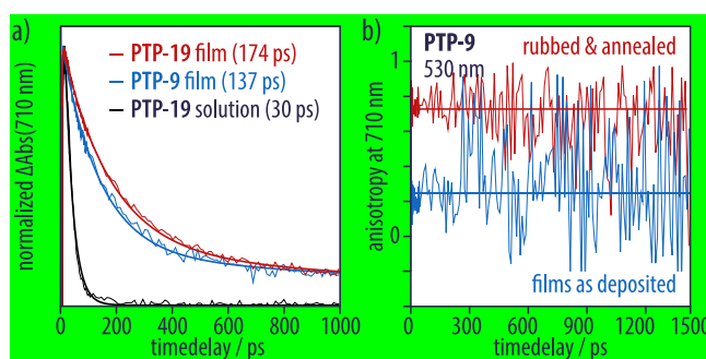
Figure 12. a) Comparison of the TA dynamics at 710 nm and the corresponding fit after excitation at 530 nm; recombination was much slower in films compared to solutions, and films made from PTP-19 showed a slower recombination as compared to PTP-9 . b) Anisotropy calculated for PTP-9 at 710 nm after excitation at 530 nm; aligned films showed an anisotropy well above that of non-aligned films; the stability of the anisotropy for non-aligned films suggested that charges did not travel between domains within the 1.5 ns timeframe of the experiment.
