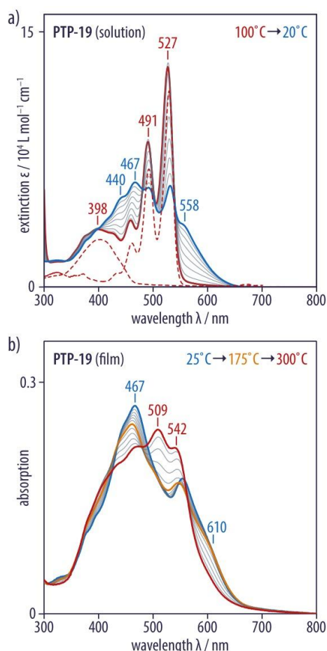
Figure 2. a) The UV/vis absorption spectrum of PTP-19 in o -dichlorobenzene ( c = 25 \mu\text{mol/L} ) at 100^\circ\text{C} (red) resembled a superposition of the contributions of perylene bisimide and quaterthiophene chromophores, as seen from a comparison to the UV/vis spectra of molecularly disperse solutions of the reference compounds 5 and 6 (red, dashed). Upon cooling the solutions from 100^\circ\text{C} to 20^\circ\text{C} (blue; in steps of 10^\circ\text{C} ), the triad formed spectroscopic aggregates, showing both H and J bands of the perylene bisimide. b) The shape of the UV/vis absorption spectra of PTP-19 in thin films remained almost unchanged upon heating from 25^\circ\text{C} (blue) to 175^\circ\text{C} (orange; in steps of 25^\circ\text{C} ), but underwent significant changes upon further heating to 300^\circ\text{C} (red; in steps of 25^\circ\text{C} ).
