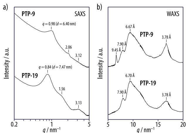
Figure 4. X-ray scattering of bulk samples of PTP-9 and PTP-19 revealed lamellar structures in the bulk. a) In the small-angle region, a reciprocal spacing ratio of q_1:q_2:q_3 = 1:2:3 and a periodicity of 6.4 nm for PTP-9 , as well as q_1:q_2:q_3:q_4 = 1:2:3:4 and 7.5 nm for PTP-19 were observed b) In the wide-angle region, the reflection at 3.78 Å was assigned to \pi - \pi stacking, and additional peaks corresponding to 7.9 and 6.7 Å were observed, of which the latter comprised at least the broad reflection associated with the short range order of the poly(isobutylene). The reflection at 9.45 Å for PTP-9 probably originates from an impurity.
