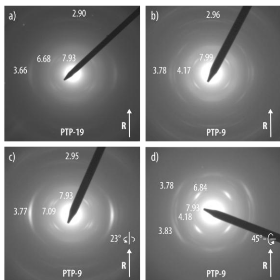
Figure 7. Electron diffraction patterns of aligned films (annealed at 300°C) obtained by high-temperature rubbing. a) PTP-19 showed reflections at 7.93, 6.68, and 3.66 Å corroborating the distances observed in X-ray diffraction. This pattern is characteristic of standing lamellae. b) The diffraction pattern of PTP-9 is dominated by a set of sharp reflections characteristic of the flat-on lamellae. The most intense reflection is observed at 7.99 Å. c) The diffraction pattern obtained by tilting the PTP-9 sample grid by an angle of \pm 23^\circ around the rubbing axis R showed the intense 3.77 Å reflection corresponding to the \pi -stacking distance between triad molecules. d) The diffraction pattern obtained by tilting the PTP-9 sample grid by an angle of \pm 45^\circ around the axis perpendicular to the rubbing axis R showed two bands at around 3.8 Å.
