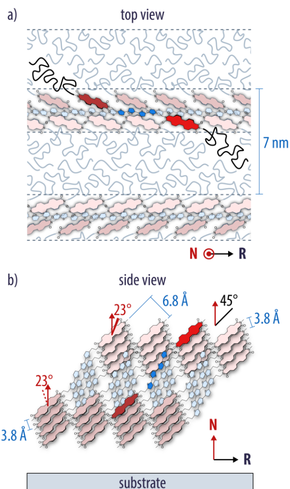
Figure 8. Schematic illustration of the molecular packing in the lamellar structure according to electron diffraction; a) top view of the lamellae (polymer segments not drawn to scale), b) side view of the triad in a lamella (attached polymer segments omitted for clarity); the triad cores are, on average aligned with their long axes parallel to the rubbing direction R ; according to the ED experiments with a tilting stage, they have an inclination of 45^\circ relative to the direction normal to the substrate N , and the \pi -conjugated planes (supposedly, of the perylenes) have an angle of \pm 23^\circ relative to N in a plane perpendicular to R .
