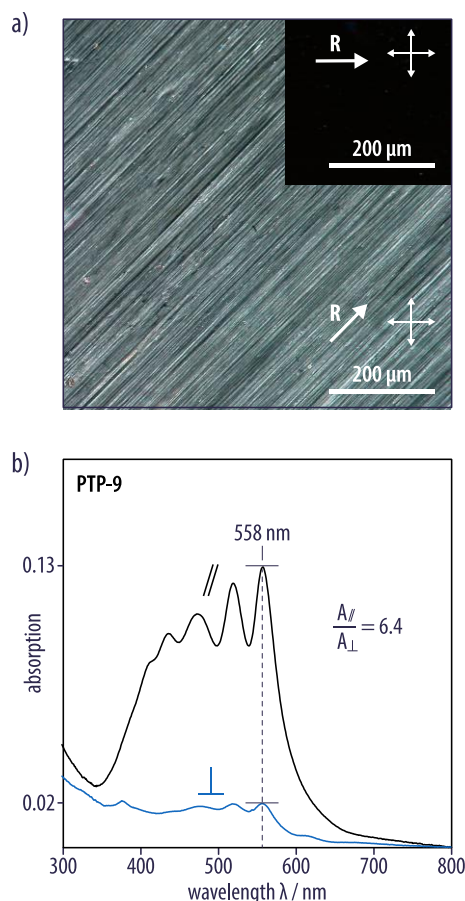
Figure 3. Aligned thin films of PTP-9 showed birefringence and dichroism. a) Polarized optical micrographs showed a strong birefringence when the rubbing direction R (white arrow) was oriented at 45° relative to the crossed polarizers, and no transmission when the rubbing direction R was perpendicular to one of the polarizers (inset). b) Polarized UV/vis spectra revealed an absorption maximum at 558 nm with a maximum intensity when the incident light was parallel to the rubbing direction.
