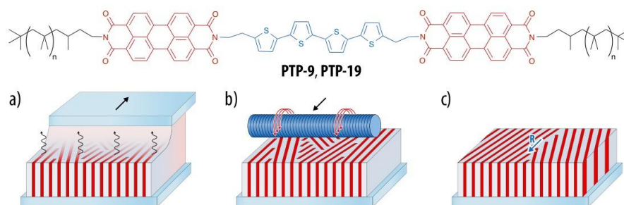
Figure 1. Molecular structure of the polymer-substituted donor-acceptor-donor triads and preparation of thin films. a ) Thin films of PTP-9 or PTP-19 ( n = 9 or 19 , respectively) were prepared by doctor blading and exhibited a lamellar phase with an “edge-on” orientation of the lamellae relative to the substrate and different lateral orientations. b ) Mechanical rubbing and annealing resulted in c ) a macroscopic alignment of the lamellar phase parallel to the rubbing direction.
