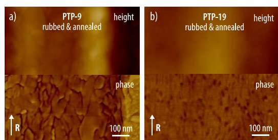
Figure 6. AFM imaging confirmed the lamellae were oriented a) face-on for PTP-9 and b) edge-on for PTP-19 . Rubbing direction R is vertical in both cases. Color scale range are a) 140 nm and 90°, and b) 150nm and 50°.
