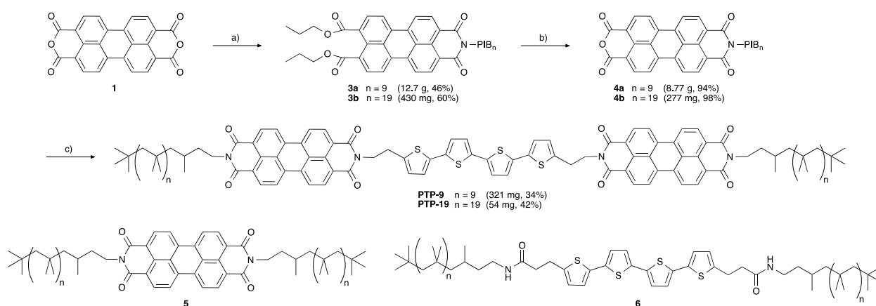
Scheme 1. Synthesis of the poly(isobutylene)-substituted triads PTP-9 and PTP-19 . Reagents and conditions: a) (i) propanol, DBU, DMF, r.t., 16h; (ii) PIB-NH 2 2a or 2b , THF, r.t., 3 d; (iii) bromopropane, r.t., 16 h; b) TsOH · H 2 O, toluene, 95^\circ\text{C} , 16 h; c) 2,5'''-bis(2-amino-ethyl)-5,2':5'',2'':5''',2'''-quaterthiophene, \text{Zn}(\text{OAc})_2 , quinoline, 175^\circ\text{C} , 16 h.
