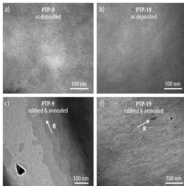
Figure 5. Transmission electron microscopy on thin film samples of PTP-9 and PTP-19 revealed stripes or terraces that were attributed to lamellae oriented edge-on or face-on relative to the substrate. a) Films of PTP-9 deposited by doctor-blading revealed stripes with a periodicity of about 7 nm. b) doctor-bladed films of PTP-19 showed a higher degree of long range order. c) Upon rubbing and annealing films of PTP-9 , the lamellae changed their orientation to a face-on orientation, resulting in terraces (annealing temperature 300°C). d) This reorientation did not occur for PTP-19 with longer side chains, which still showed stripes aligned by the rubbing process (annealing temperature 270°C). The rubbing direction R is indicated by the white arrow.
