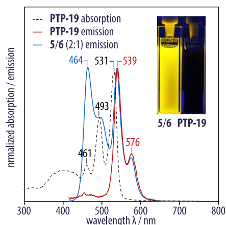
Figure 9. The emission spectrum (upon excitation at 400 nm) of PTP-19 (red) was identical to the emission of the perylene 5 (not shown). However, compared to the mixture 5/6 (2:1) with the same composition of the individual chromophores (blue), fluorescence was quenched by more than 99% (inset). In comparison with the mixture, the absence of quaterthiophene emission feature in the emission of the triad PTP-19 suggested an energy transfer to the perylene moiety.
