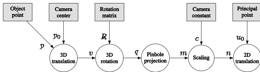
Figure 1: The computational chain corresponding to equation (5). The grey rectangles indicate bundle adjustment parameters. The white circles indicate component functions from equation (4). The arrows indicate how the parameters and results are propagated. The arrow labels indicate the name of the formal (input) parameter of the corresponding function.
