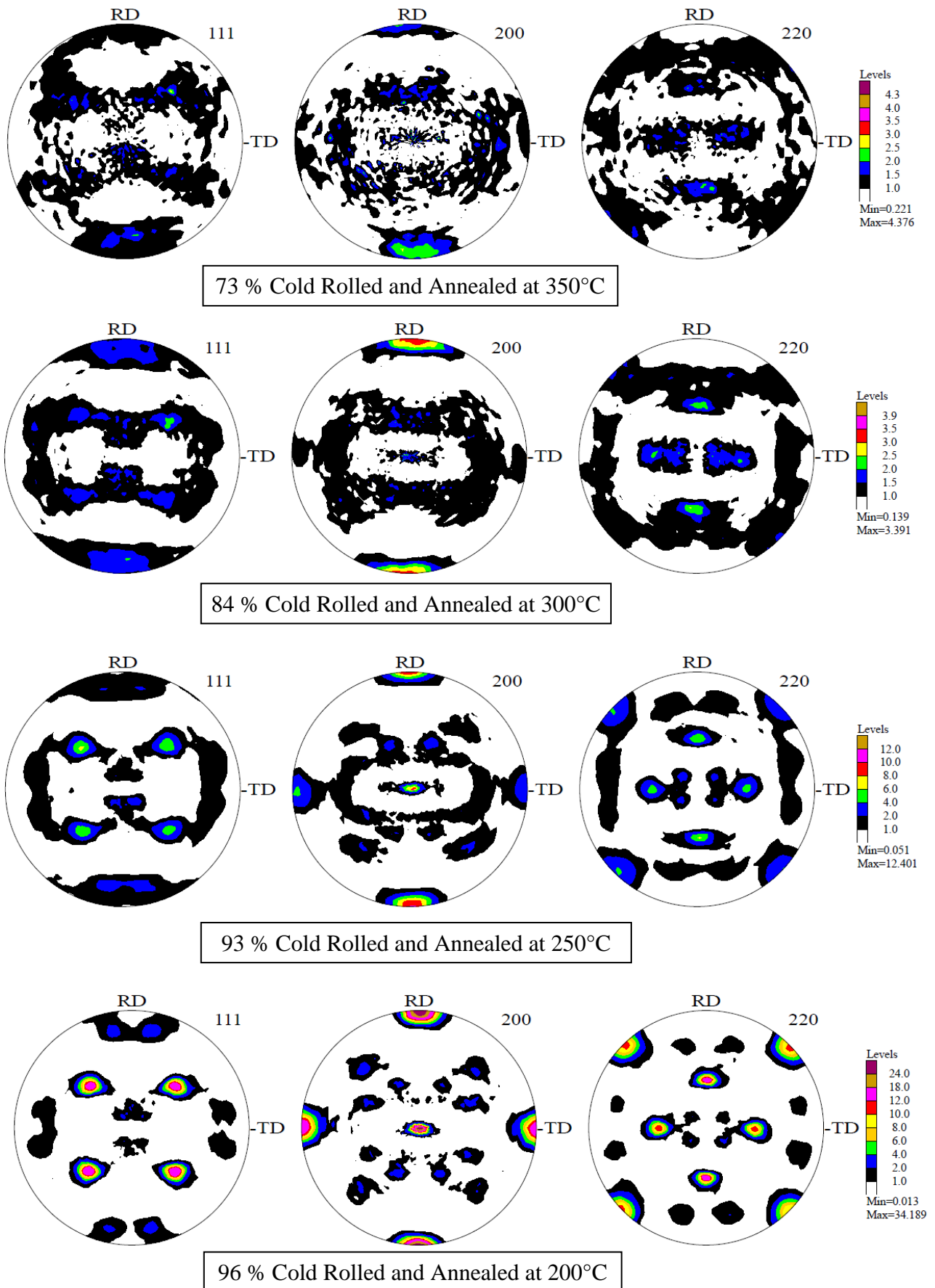
Fig. 2. (111), (200) and (220) recalculated pole figures, measured by X-ray diffraction after different amounts of cold – rolling, followed by a heat-treatment inducing full recrystallization.
