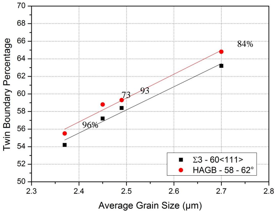
Fig. 6. Evolution of the Twin Boundary percentage as a function of the average grain size. Two different descriptions have been selected for the twin boundaries: these are described by a rotation of 60^\circ around a \langle 111 \rangle axis (CSL description, tolerance angle of 5.8^\circ ) (black symbols) or by a HAGB associated with an angle varying between 58^\circ and 62^\circ (red symbols).
