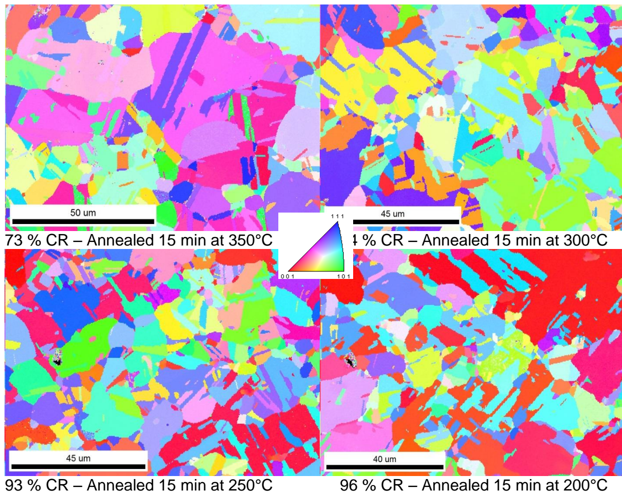
Fig. 4. Typical EBSD orientations maps obtained for the 4 investigated materials. The color indicates the orientation of the rolling direction of the sample, according to the color code indicated by the small triangle. The step size is 0.3 \mu\text{m} .
