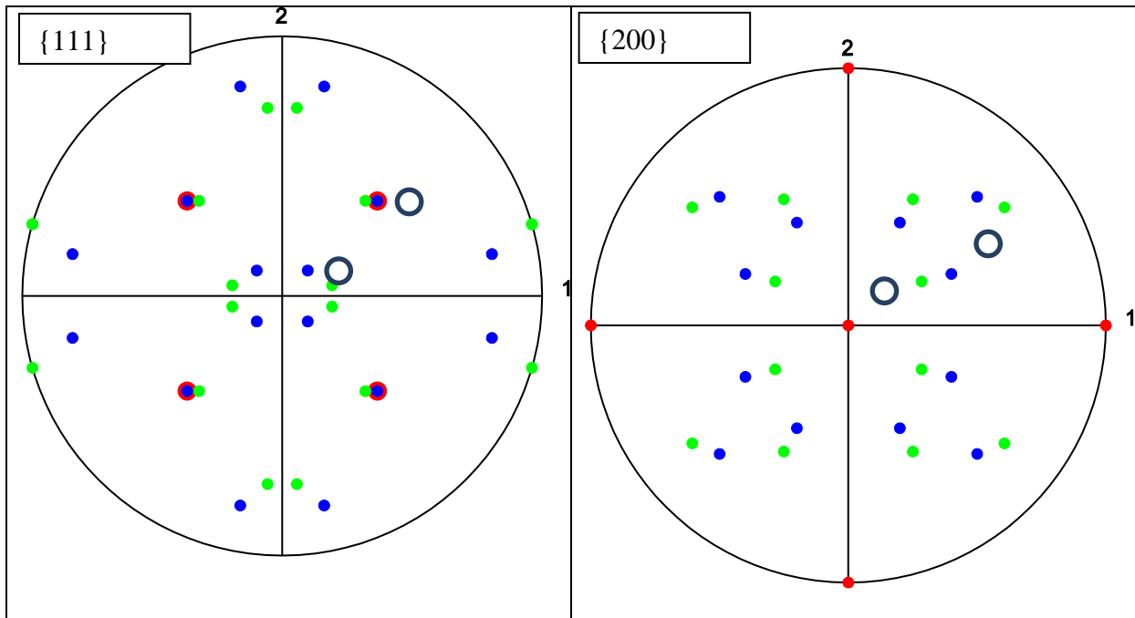
Fig. 11. Calculated pole figures indicating the positions of the \{111\} poles (left) and \{200\} poles (right) for the orientations Cube (in red), Twinned Cube (in blue) and S (in green). Open grey circles: measurement points. 1 = RD (rolling direction).
