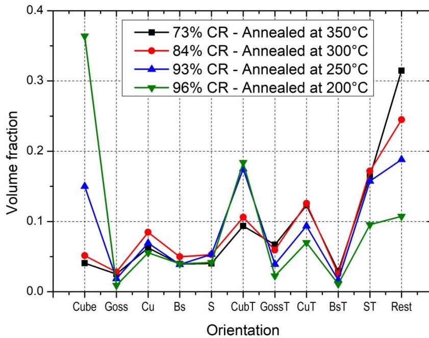
Fig. 3. Calculated volume fractions from the XRD measurements of the principal texture components and associated twin components classically composing the rolled and annealing copper textures. The symmetrical orientations (due to the orthotropy of the rolling process) are grouped, as well as the different twin orientations associated with one given orientation. Rest is composed of all remaining orientations present in the texture which are not closed to one of the 50 orientations of interest.
