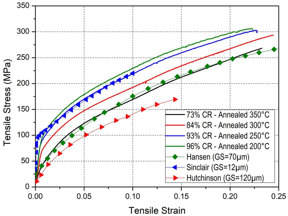
Fig. 9. Experimental tensile curves obtained after the 4 thermomechanical treatments; some other tensile curves extracted from the literature are also added for comparison. The numbers in brackets indicate the average grain size (GS) of the samples, usually determined by optical microscopy, without considering the twinned parts of the grains.
