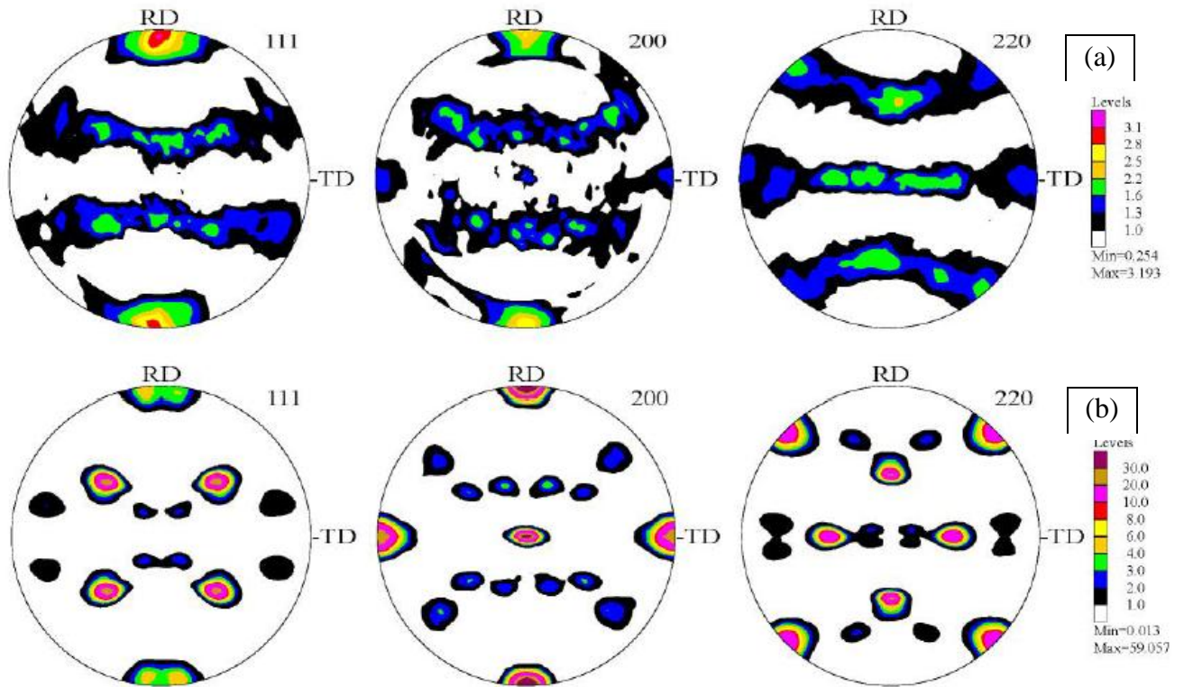
Fig. 8. Recalculated pole figures, measured by X-ray diffraction after 25% plastic strain for the two samples subjected to the two extreme thermomechanical processes : (a) 73% CR + annealing at 350°C during 15 minutes and (b) 96% CR + annealing at 200°C during 15 minutes.
