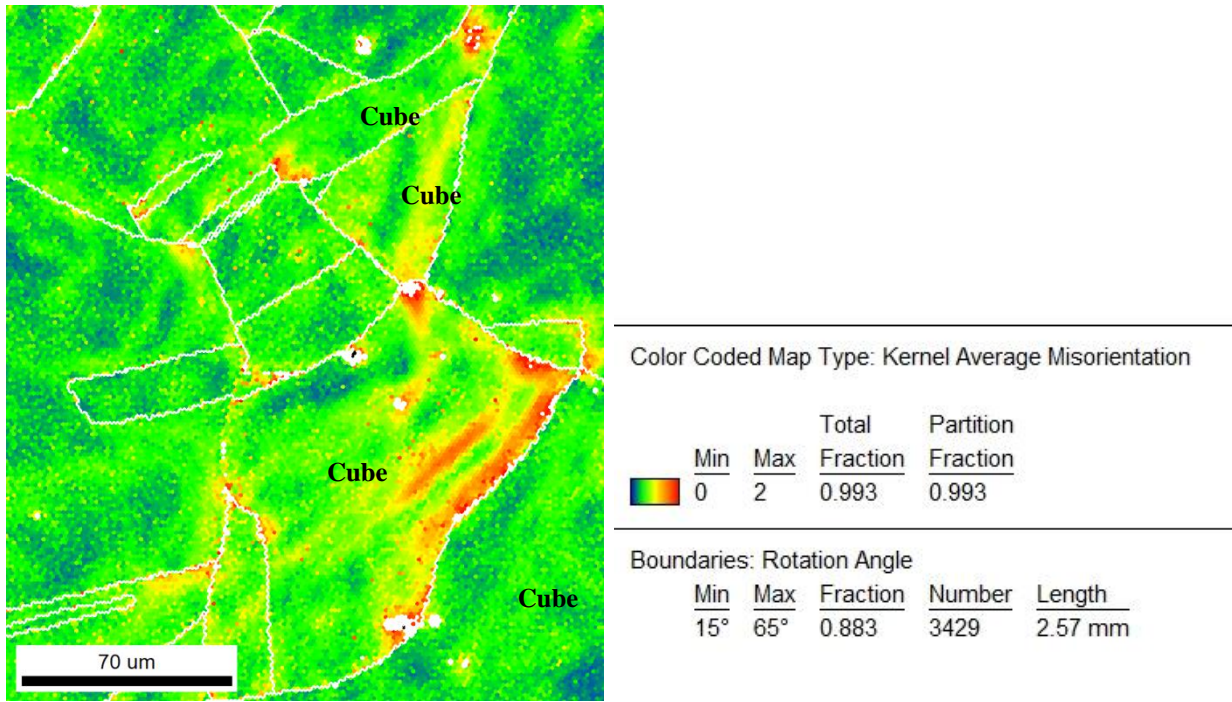
Fig. 13. EBSD map measured after 20% plastic strain for an isotropic Cu sample [45]. The color code indicates the value of the local KAM parameter between 0 and 2°.
