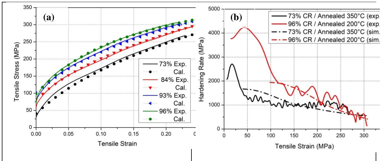
Fig. 14. Comparison of experimental and predicted plastic parts of the tensile curves (a) and hardening rates for the two extreme cases (b).
