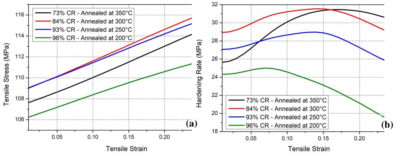
Fig. 17. Tensile (a) and hardening (b) curves, predicted by considering constant CSSs (and associated dislocation densities).
