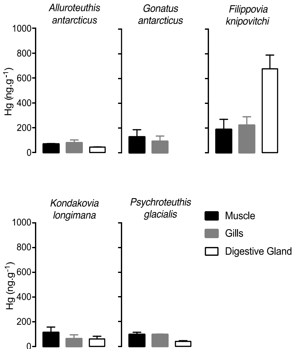
Figure 3. Total mercury concentrations (Mean \pm SD, \text{ng g}^{-1} dw) in different tissues (muscle, gills and digestive gland) of Antarctic squid collected around South Georgia in the austral summer of 2012/2013. No digestive gland tissue was available for G. antarcticus .
