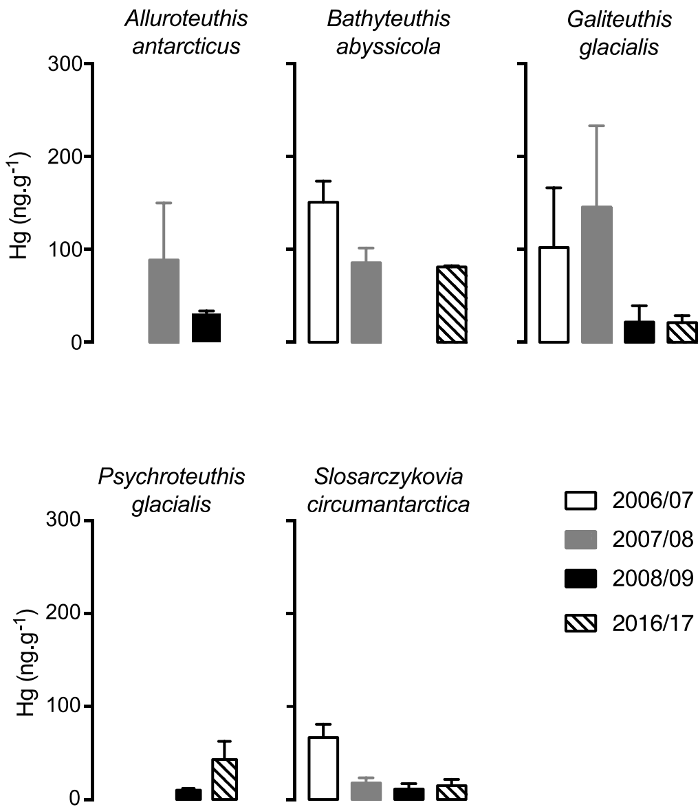
Figure 4. Total mercury concentrations (Mean \pm SD, ng g -1 dw) in the muscles of Antarctic squid from the Southern Ocean collected around South Georgia in the austral summers of 2006/07, 2007/08, 2008/09 and 2016/17.
