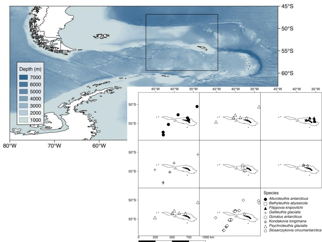
Figure 1. Sampling sites and distribution of species captured around South Georgia across all sampling years. Lines represent 1000m isobath.
