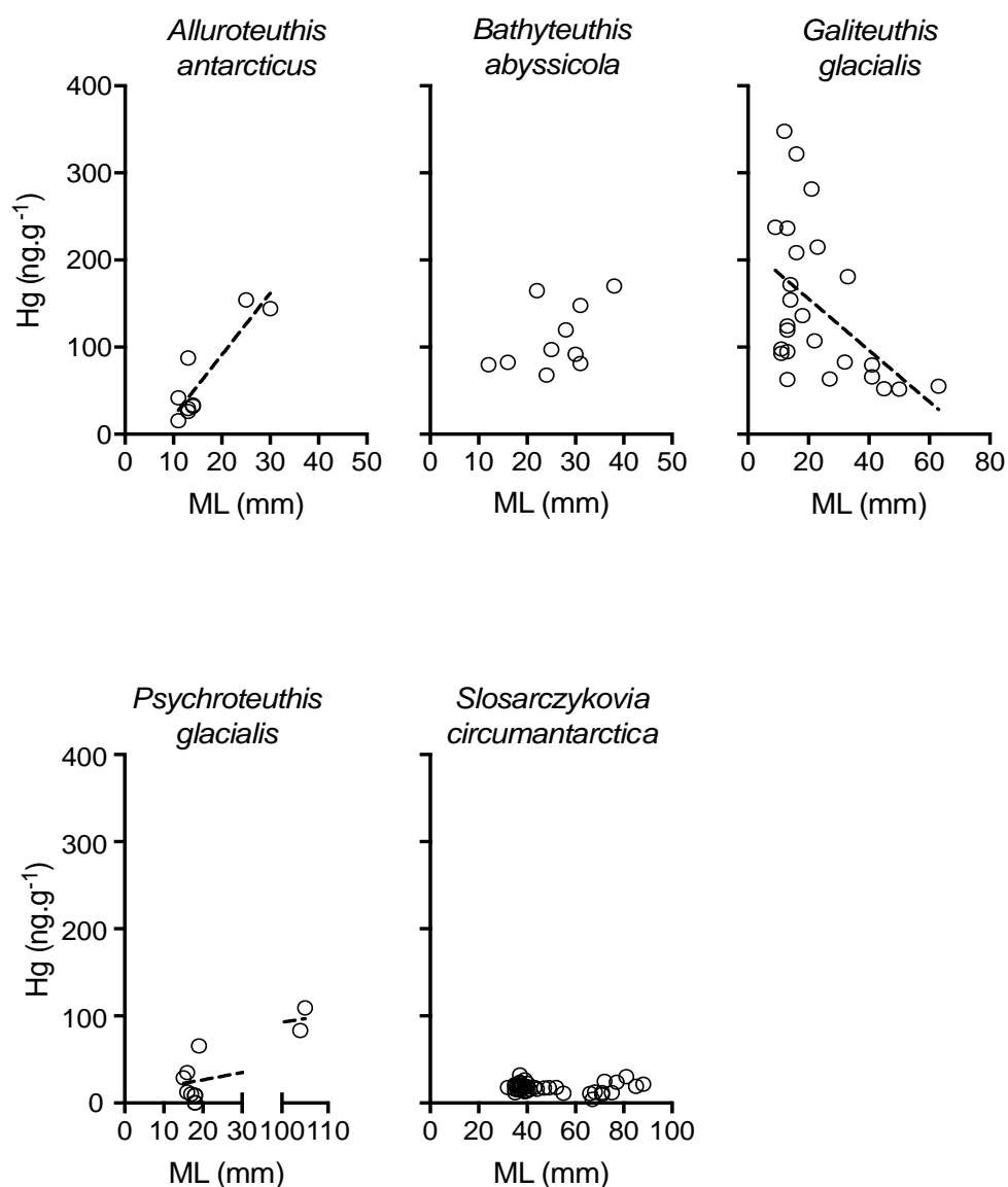
Figure 2. Total mercury concentration ( \text{ng g}^{-1} \text{ dw} ) versus mantle length (ML; mm) in individual Antarctic squid collected around South Georgia in the austral summer of 2007/08 (except Psychroteuthis glacialis 2016/17). Regression equations are given in the text.
