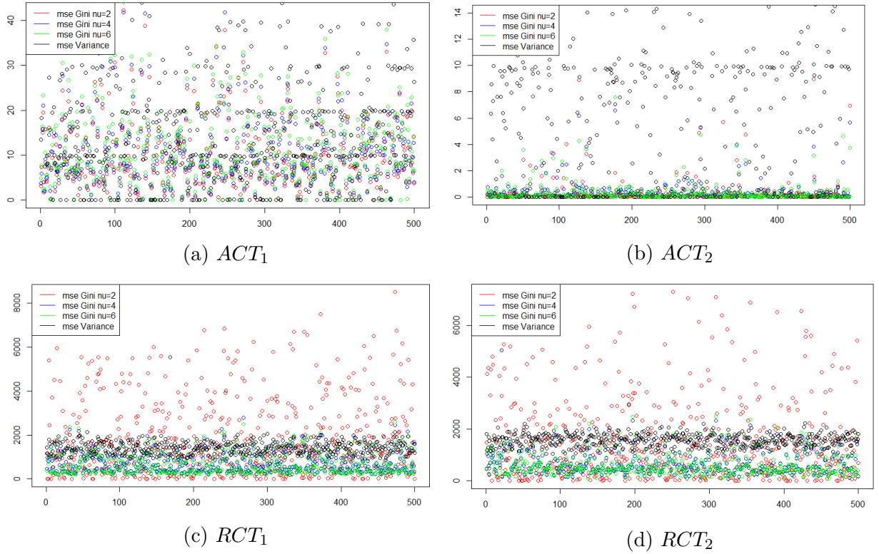
Figure 4: ACT_1 , ACT_2 , RCT_1 and RCT_2
