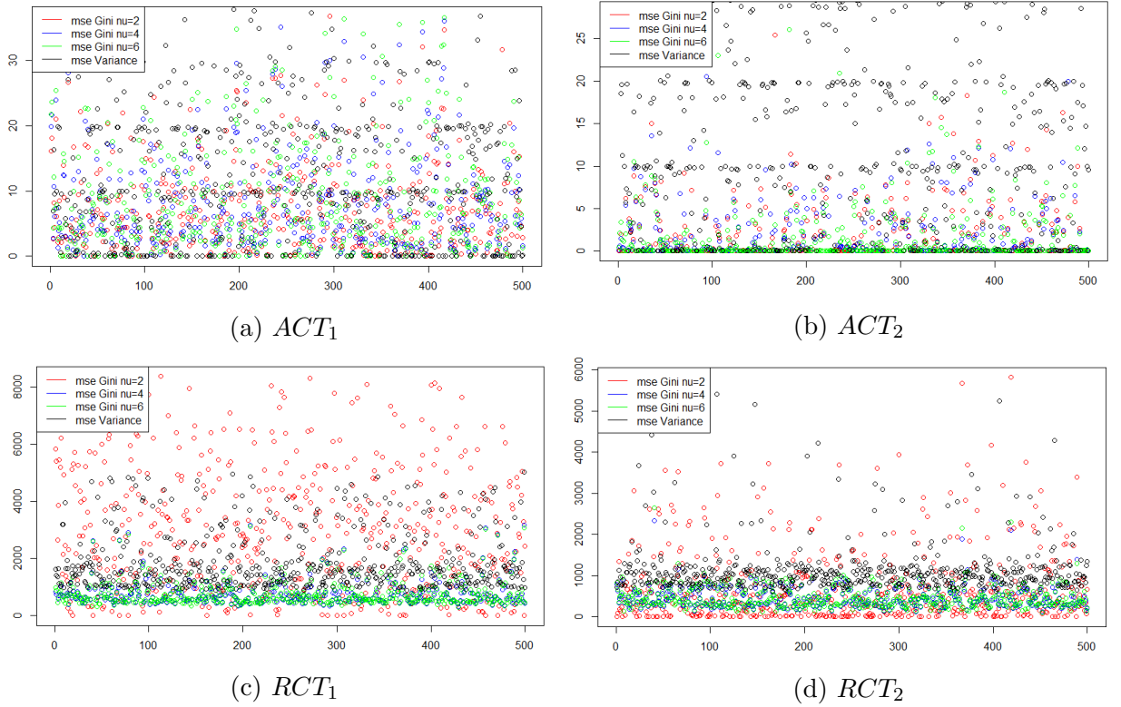
Figure 3: ACT_1 , ACT_2 , RCT_1 and RCT_2
