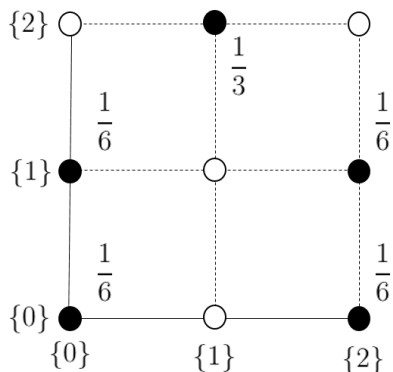
Figure 1: Joint distribution of a random pair (X_k, X_\ell) such that \mathbb{E}[X_k h(X_\ell)] \neq \mathbb{E}[X_\ell h(X_k)] , with non-exchangeable components X_k \stackrel{\mathcal{L}}{=} X_\ell .
