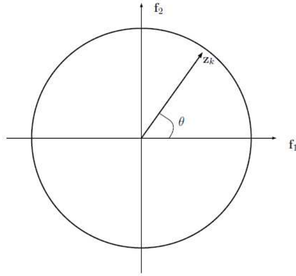
Figure 2: Circle of correlation
