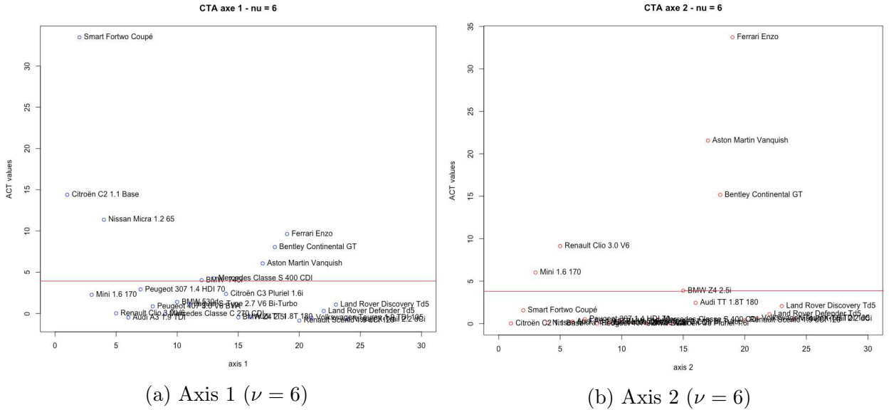
Figure 10: Gini ACTs ( \nu = 6 )
