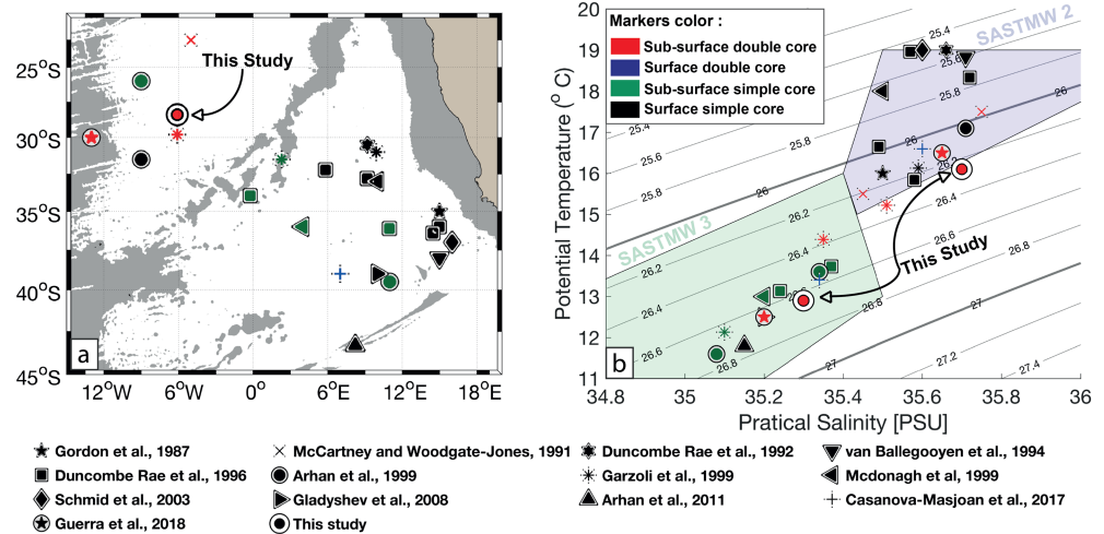
Figure 16. (a) Position and (b) hydrological properties in the mode water cores of the Agulhas Rings described in the literature. Each study discussing one or more of these eddies is associated with a specific marker, and the color corresponds to a particular type of eddy. Double-core mode water eddies have two similar markers. The gray shaded patches in (a) represent water depth shallower than 3,500 m in the ETOPO2 data set (Smith & Sandwell, 1997). The background lines in (b) represent isopycnals of potential density anomalies referenced to the surface pressure ( \sigma_0 ). The blue and green shaded patches highlight the hydrological properties of, respectively, SASTMW2 and SASTMW3 as described by Sato and Polito (2014).
