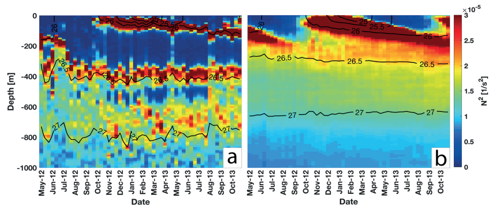
Figure 7. Time evolution of the Brunt Väisälä frequency squared ( N^2 ) computed for the Argo float No. 5902281 profiles (a) within the Agulhas Ring, and (b) for the environment climatology. Isopycnal levels separated by a 0.5 \text{ kg}^{-3} interval are added to the corresponding panels.
