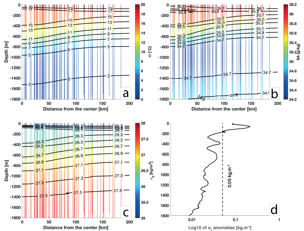
Figure 11. Superposition of the observed (background color) and the reconstructed (black contours) Agulhas Ring of the (a) conservative temperature ( \Theta ), (b) absolute salinity (SA), (c) potential density ( \sigma_0 ), and (d) root-mean-square error between the observed \sigma_0 anomalies and the reconstructed values computed at each depth.
