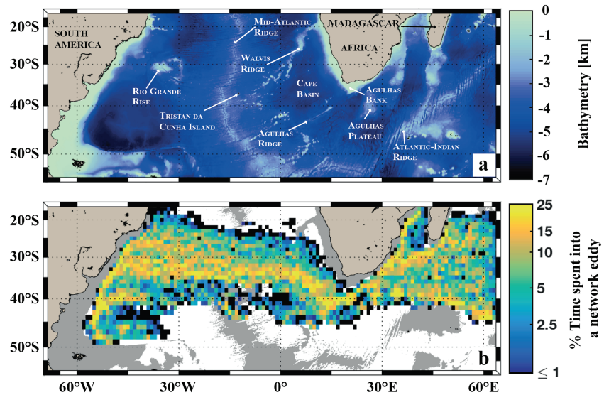
Figure 1. The study domain presented in terms of (a) the local bathymetry from the ETOPO2 data set (Smith & Sandwell, 1997) and (b) the percentage of time each 2^\circ \times 2^\circ grid cell is occupied by the core of an eddy occurrence as part of the Agulhas Ring Eddy Network (Laxenaire et al., 2018). Figure modified from Laxenaire et al. (2018).
