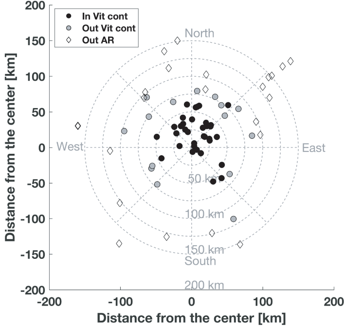
Figure 10. Position of the Argo profiles in the moving frame of the Agulhas Ring. The center of the frame corresponds to the centroid of the characteristic eddy contour delimited by R_{Vmax} and computed from ADT maps. The filled circles indicate Argo profiles inside the characteristic eddy contour, the gray circles those inside outer eddy edge, and the empty diamond those outside the Agulhas Ring and any other neighboring eddy and lying at a 160 km radius from the Agulhas Ring center.
