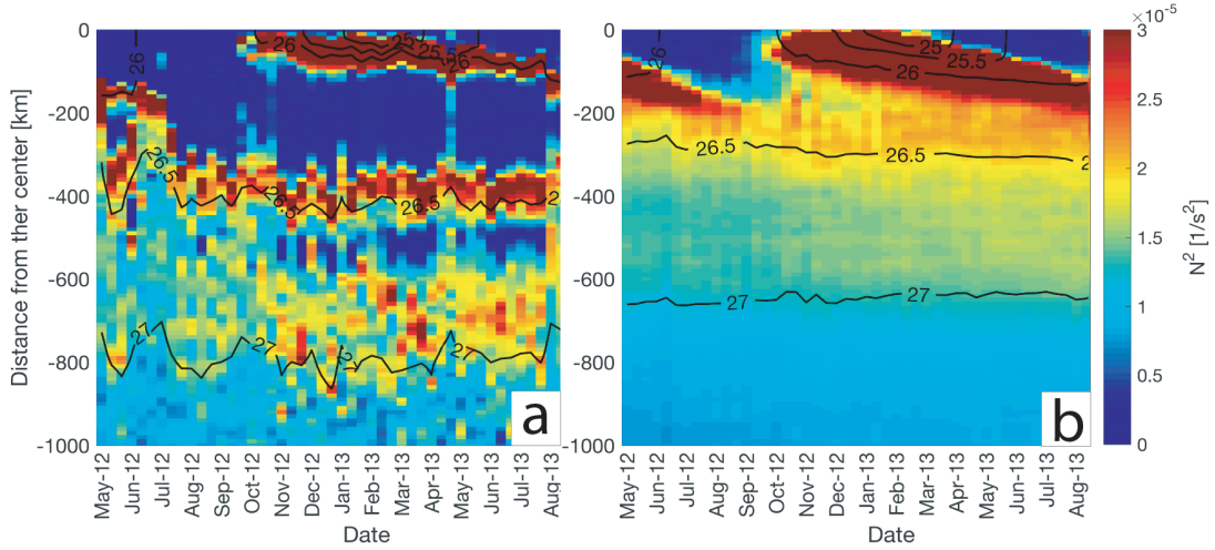
Figure 7. Time evolution of the Brunt Väisälä frequency squared computed for the Argo float No. 5902281 profiles a) within the Agulhas Ring, and b) for the environment climatology. Isopycnal levels separated by a 0.5 \text{ kg}^{-3} interval are added to the corresponding panels.
