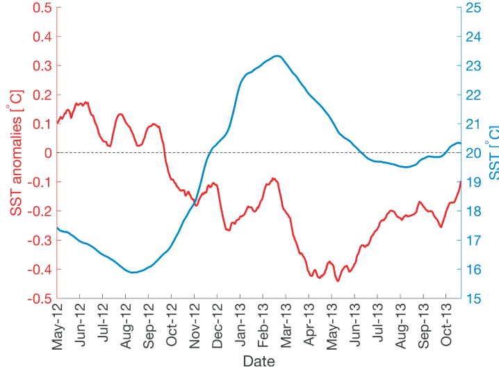
Figure 8. Sea Surface Temperature (blue) and associated anomalies (red) interpolated from the ODYSSEA SST dataset (Dash et al., 2012; Martin et al., 2012) at the center of the Agulhas Ring. The anomalies are computed by subtracting the mean SST (computed as the average of the SST in the square box area of 300 km×300 km centered on the eddy center) to the SST value in the center of the eddy. All the data were smoothed by a moving average associated with a monthly window.
