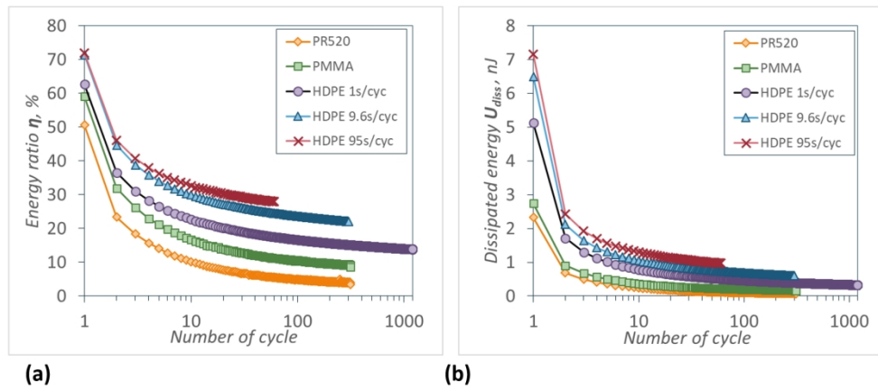
FIG. 5. (a) The energy ratio and (b) dissipated energy evolutions with cycles for PR520 epoxy, PMMA and HDPE at three loading rates. <<color online>>
