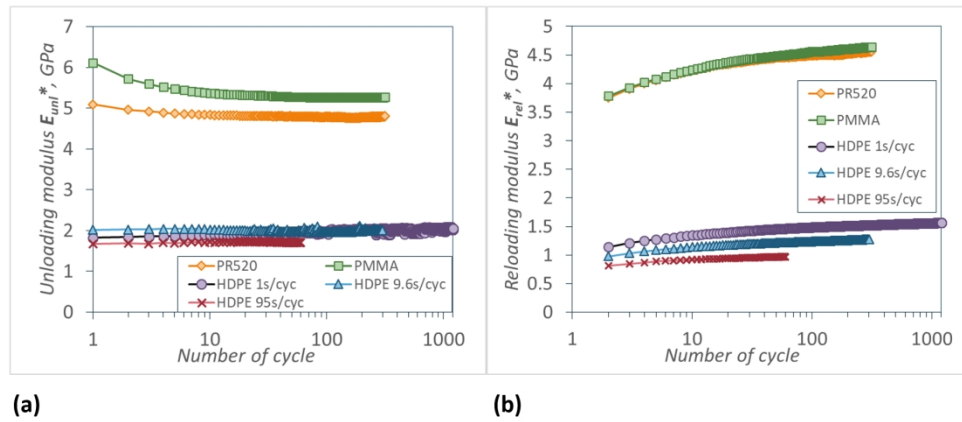
FIG. 3. (a) Unloading and (b) reloading instantaneous elastic moduli deduced from the cyclic indentation tests on PR520 epoxy, PMMA and HDPE at three loading rates. <<color online>>
