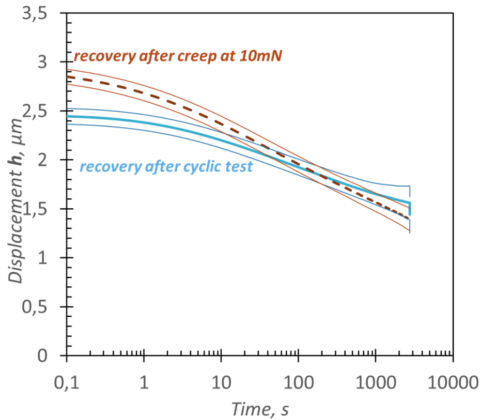
FIG. 7. Viscoelastic recovery after indentation cyclic test of 9.6 s/cyc and indentation creep test at 10 mN on HDPE. The upper and lower bounds represent variability between 9 tests. <<color online>>
