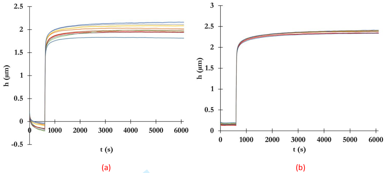
FIG. S3. Effect of the thermal drift correction procedure on long creep test on HDPE at 5 mN: (a) before the correction, (b) after the correction
