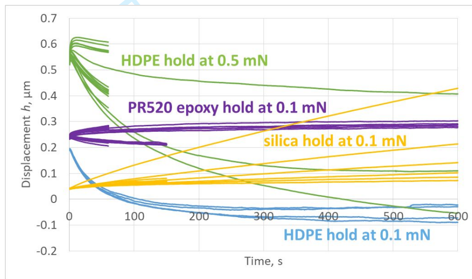
FIG. S2. Displacement drift data for load hold at 0.1 or 0.5 mN on fused silica, PR520 epoxy and HDPE without any correction.
