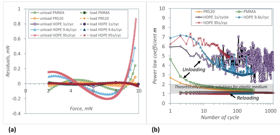
FIG. 4. (a) Plot of residuals for the first unloading and first reloading and (b) power law coefficients for the whole test of loading and unloading curves fitted with Eq. 1. <<color online>>
