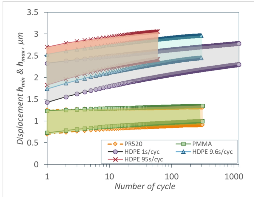
FIG. 2. Maximal and minimal displacement evolutions during indentation cycling of PR520 epoxy, PMMA and HDPE. <<color online>>
