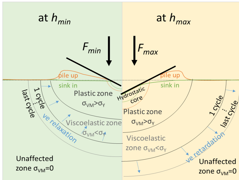
FIG. 8. Schematic distribution of Von Mises stress under the indenter at maximal displacement (on the right) and minimal displacement (on the left) with pile up (in orange) and sink in (in green) scenarios. <<color online>>
