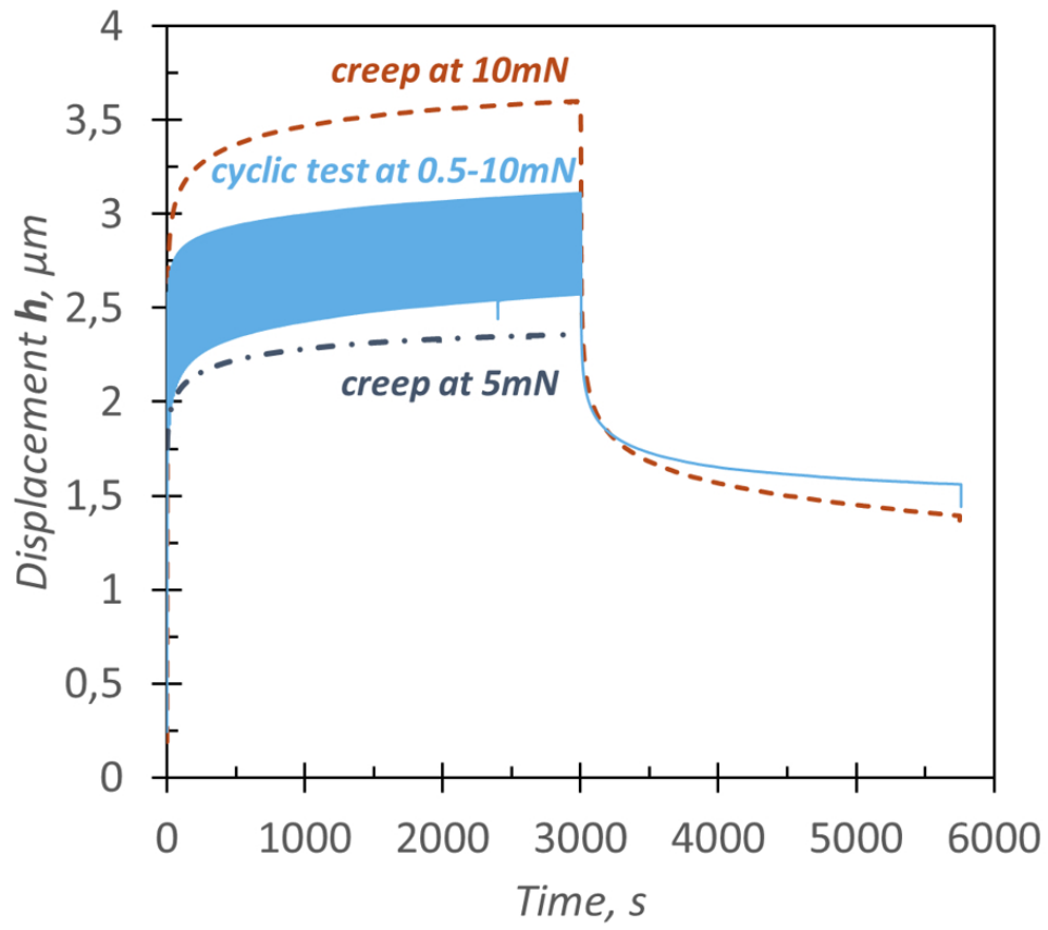
FIG. 6. Cyclic indentation test at 9.6 s/cyc and indentation creep tests at the same maximal load and a half of maximal load on HDPE. <<color online>>
