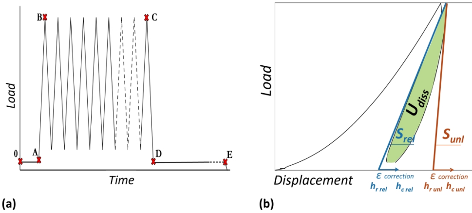
FIG. 1. (a) Loading path of the cyclic indentation test and (b) schematic of the cycle analysis. <<color online>>
