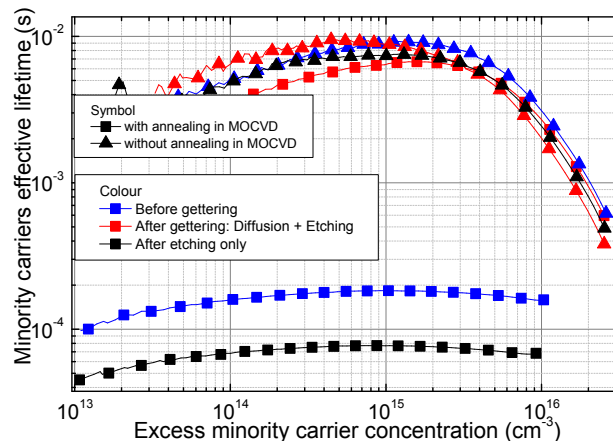
Fig. 5. Minority carrier lifetime for silicon wafers after annealing in the MOCVD chamber, and after phosphorous diffusion and/or etching. The minority carrier lifetime is also reported for a reference wafer without annealing.
