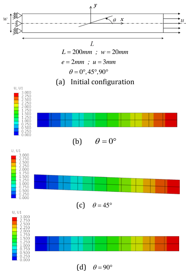
Figure 4 Unidirectional tensile tests: Finite element simulation for different fiber orientation ((a): Initial configuration; (b): \theta = 0^\circ ; (c): \theta = 45^\circ ; (d): \theta = 90^\circ ).
