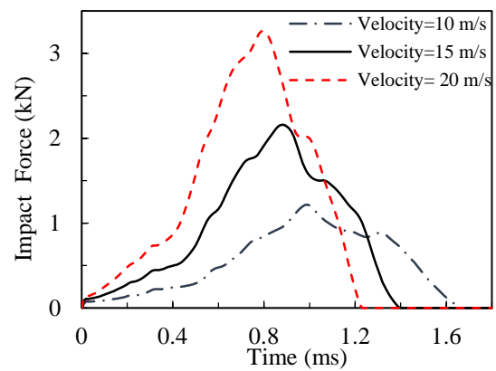
Figure 18 Impact force versus time responses for e=1 mm, R_p=6.35 mm and m_p=54.4 m/s.
