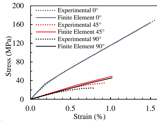
Figure 5 Uniaxial tensile tests at 0°, 45° and 90°, present finite element results versus experimental results from Cherif et al. [8].
