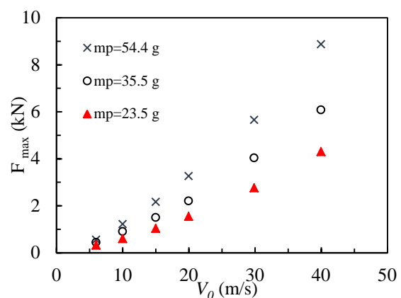
Figure 19 Maximum impact force versus initial impactor velocity.
