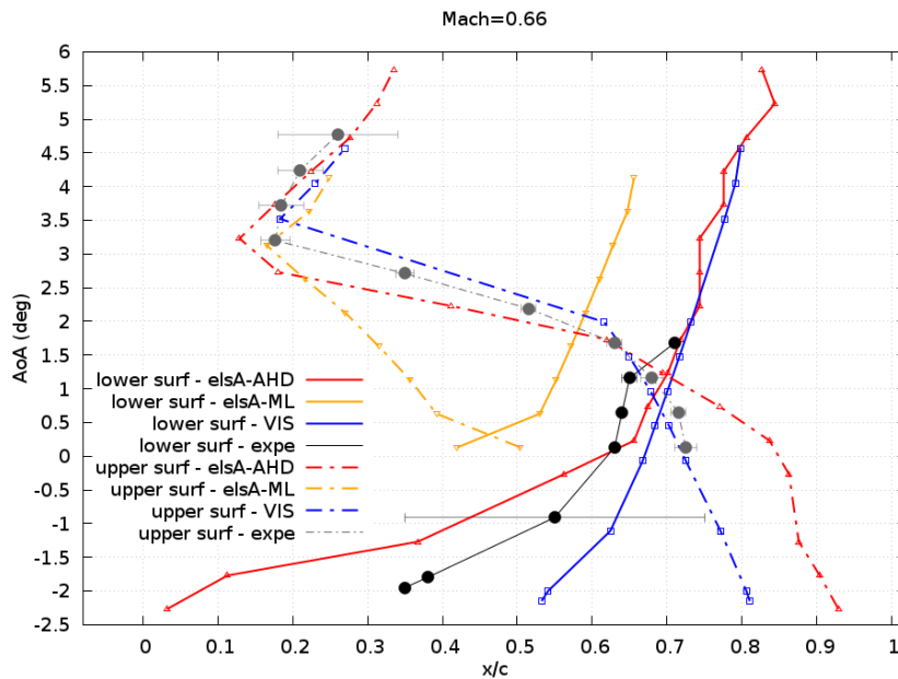
Figure 3: Evolution of the transition location against the angle of attack
