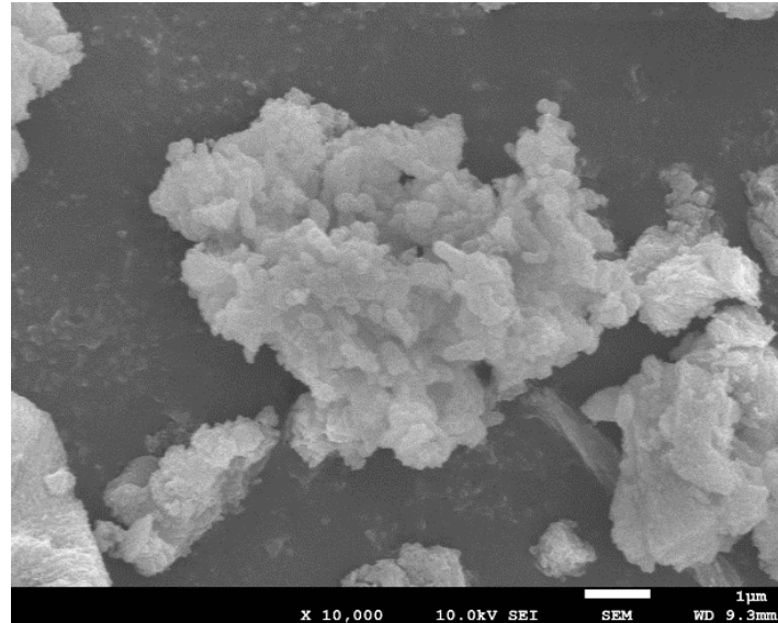
Figure 4. SEM imaging of \text{Ca}(\text{OH})_2 particles.
