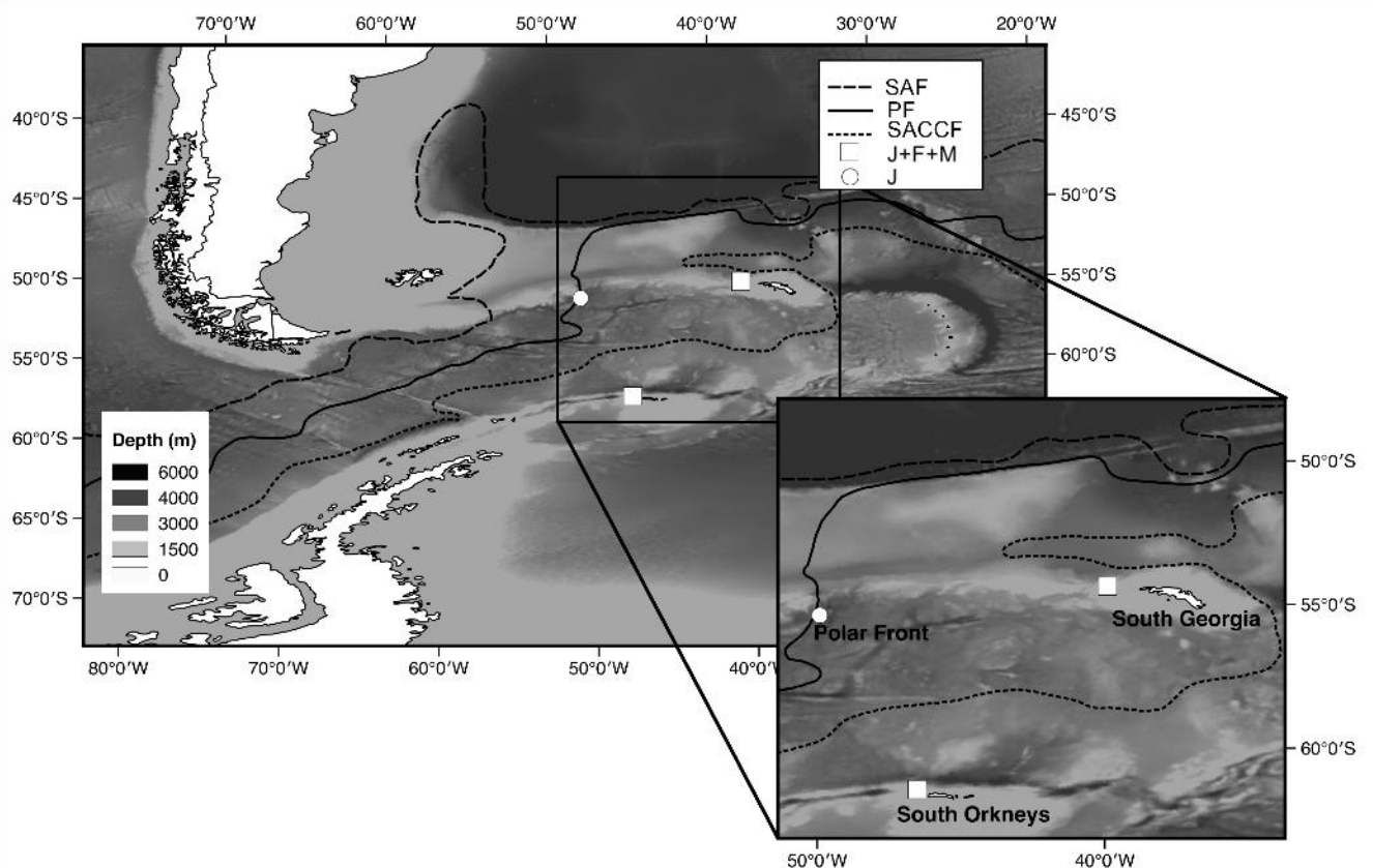
Figure 1 – Sampling sites of Antarctic krill (white square – samples of juveniles, females and males; white dot – samples of juveniles ) and general positions of the
