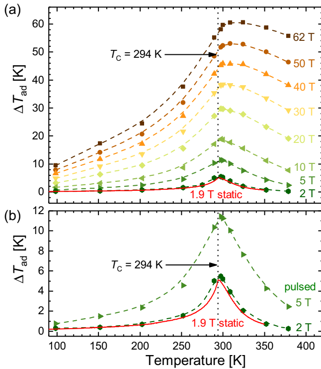
FIG. 3. (a) Adiabatic temperature change \Delta T_{ad} as a function of temperature for different magnetic fields. The data points were extracted from the magnetic-field dependencies of \Delta T_{ad} for given field values. They are connected with dashed lines as a guide to the eye. The solid line shows the data obtained from direct measurements of the adiabatic temperature change under quasistatic conditions. (b) The low-field region of (a).
