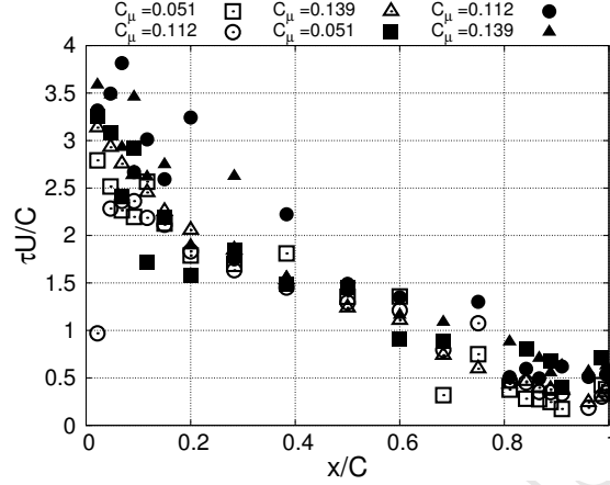
Figure 12: Distribution of the time responses \tau with the chord for varying actuation intensity at \alpha = 0 . Open and closed symbols are for opening and closing actuation respectively
