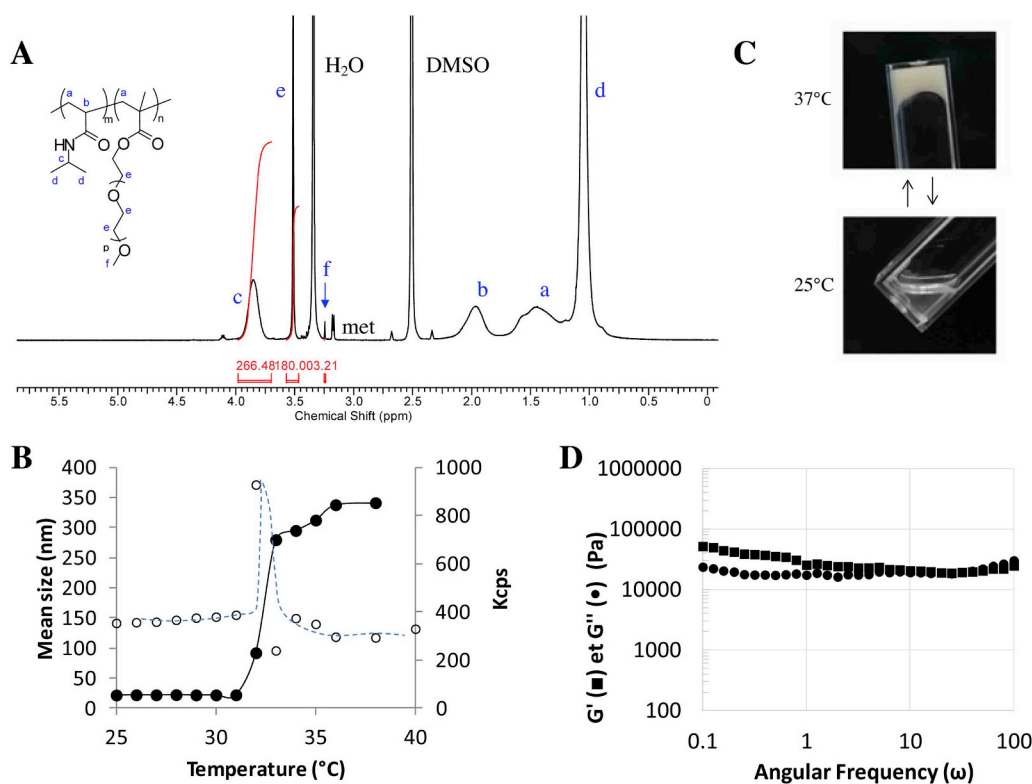
Fig. 1. Hydrogel preparation and characterization. A. ^1\text{H} NMR of the PNIPAAm-g-PEG copolymer in \text{DMSO-}d_6 (met. = methanol traces; -\text{C-CH}_3 and -\text{CH}_2\text{-OC(O)-} protons from the original PEGMA are overlapped); B. LCST of the copolymer determined by DLS (PBS, pH 7.4); C. Hydrogel formation at 37^\circ\text{C} (13.7 wt% in PBS, pH 7.4); D. Storage modulus ( G' ) and loss modulus ( G'' ) of the copolymer hydrogel (13.7 wt% in PBS, pH 7.4) at 37^\circ\text{C} .
