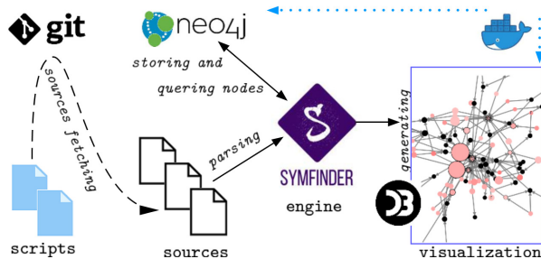
Figure 2: The dockerized symfinder toolchain
