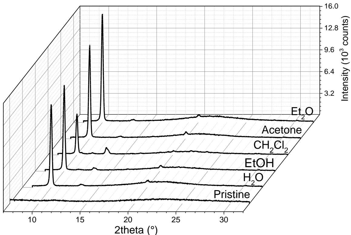
Figure 1. XRD patterns of [\text{Fe}(\text{HB}(\text{tz})_3)_2] thin films exposed to different solvents. The diffractogram of a pristine film is also shown. ( N.B. The broad peak around 2\theta = 15^\circ\text{--}27^\circ is typical for amorphous fused silica substrates used in this study. 32 )
