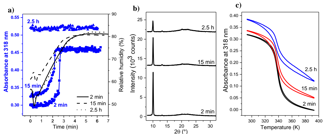
Figure 5. Investigation of three different [\text{Fe}(\text{HB}(\text{tz})_3)_2] thin films (each approx.. 100 nm thick) stored in air for 2 min, 15 min and 2.5 hours before water vapor annealing: (a) Absorbance change ( \lambda = 318 nm; baseline corrected) during water vapor annealing (i.e. for increasing the RH from the ambient value to 80 %). (b) XRD patterns and (c) temperature dependence of the absorbance (second heating–cooling cycle, \lambda = 318 nm, dT/dt = 1 K \text{min}^{-1} ; baseline corrected) following the water vapor treatment.
