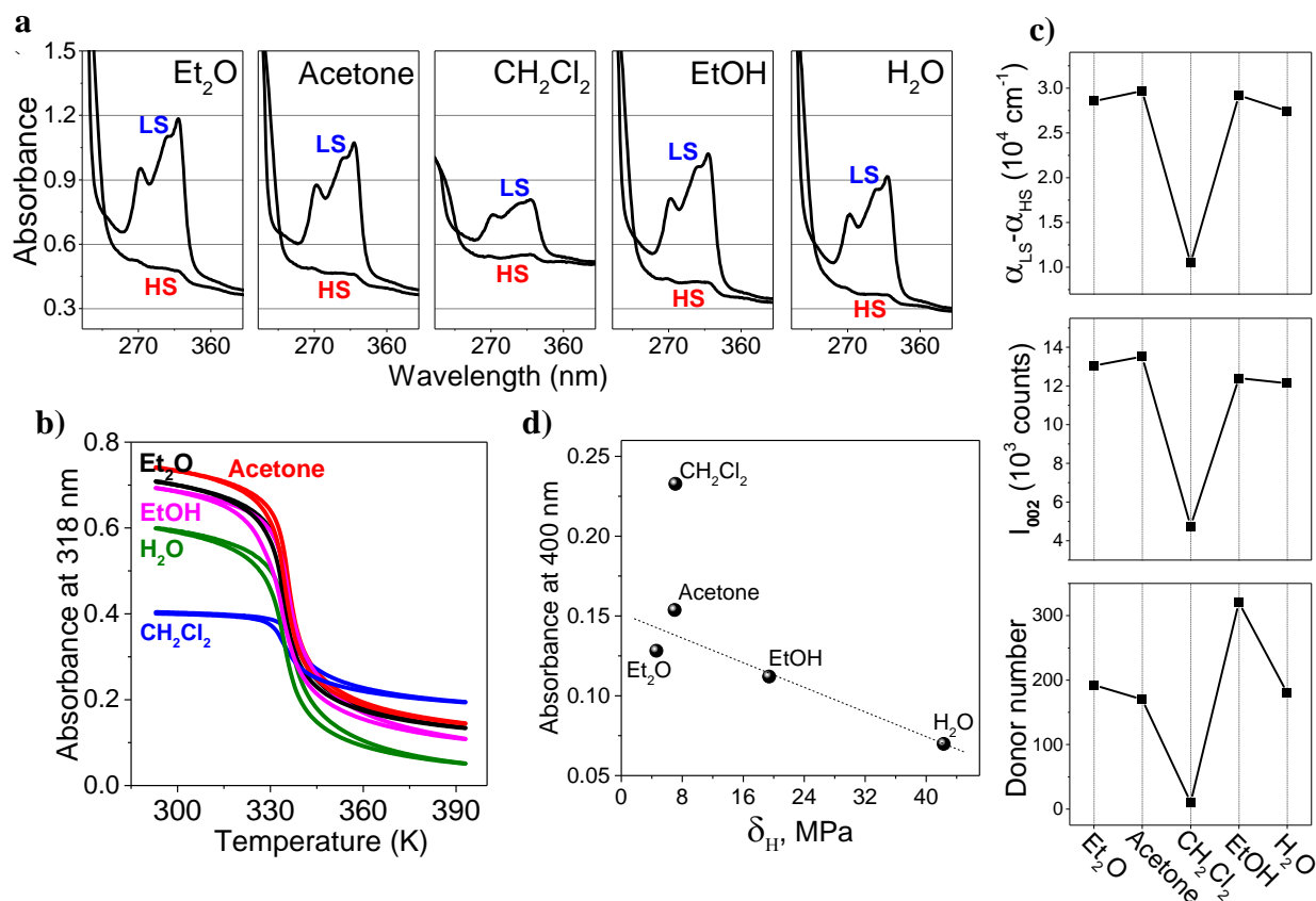
Figure 2. (a) Absorbance spectra acquired at 293 K (LS) and 393 K (HS) in the heating mode for [Fe(HB(tz) 3 ) 2 ] films annealed with different solvents (uncorrected spectra). (b) Temperature dependence of the absorbance at 318 nm (baseline corrected) along the second heating-cooling cycle recorded at 1 K min -1 scan rate for different solvent treated samples. (c) Absorbance coefficient change at the spin transition ( \lambda = 318 nm), intensity of the 002 XRD peak (thickness normalized) and solvent donor number for different solvent treated samples. (d) Absorbance at 400 nm (baseline corrected) as a function of the Hansen solubility parameter \delta_H .
