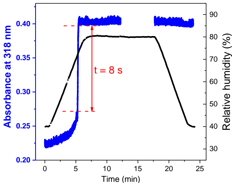
Figure 4. Absorbance change (baseline corrected) at 318 nm of a [\text{Fe}(\text{HB}(\text{tz})_3)_2] thin film as a function of time (blue curve) for increasing and decreasing values of relative humidity (black curve) at a fixed temperature of 298 K. (Note that between ca. 12.5 and 17.5 min no absorbance data were acquired.)
