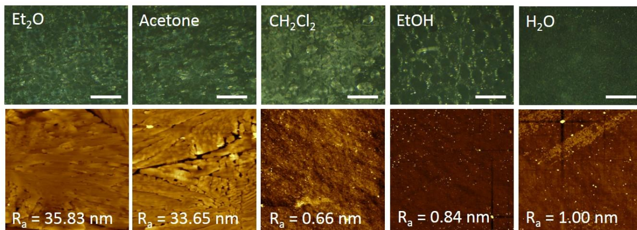
Figure 3. Optical microscopy (top panel) and AFM surface topography (bottom panel) characterization of the different solvent vapor annealed [\text{Fe}(\text{HB}(\text{tz})_3)_2] films. Scale bar in optical images: 500 \mu\text{m} ; AFM image size: 30 \times 30 \mu\text{m}^2 .
